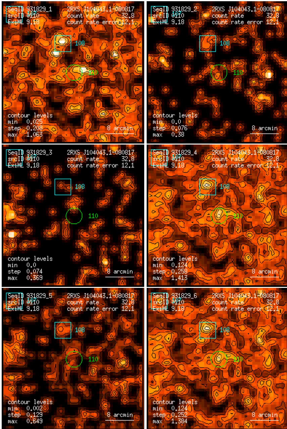
Figure 110: RASS 931829: detection 0110: band rate images, Gaussian filter: (1) PSPC channels 11 – 41, (2) 52 – 90, (3) 91 – 201, (4) 11 – 235, (5) 52 – 201, (6) 11 – 201. Broad band rates in counts/ks. Band rate contour levels in counts/ks/arcmin 2 .
