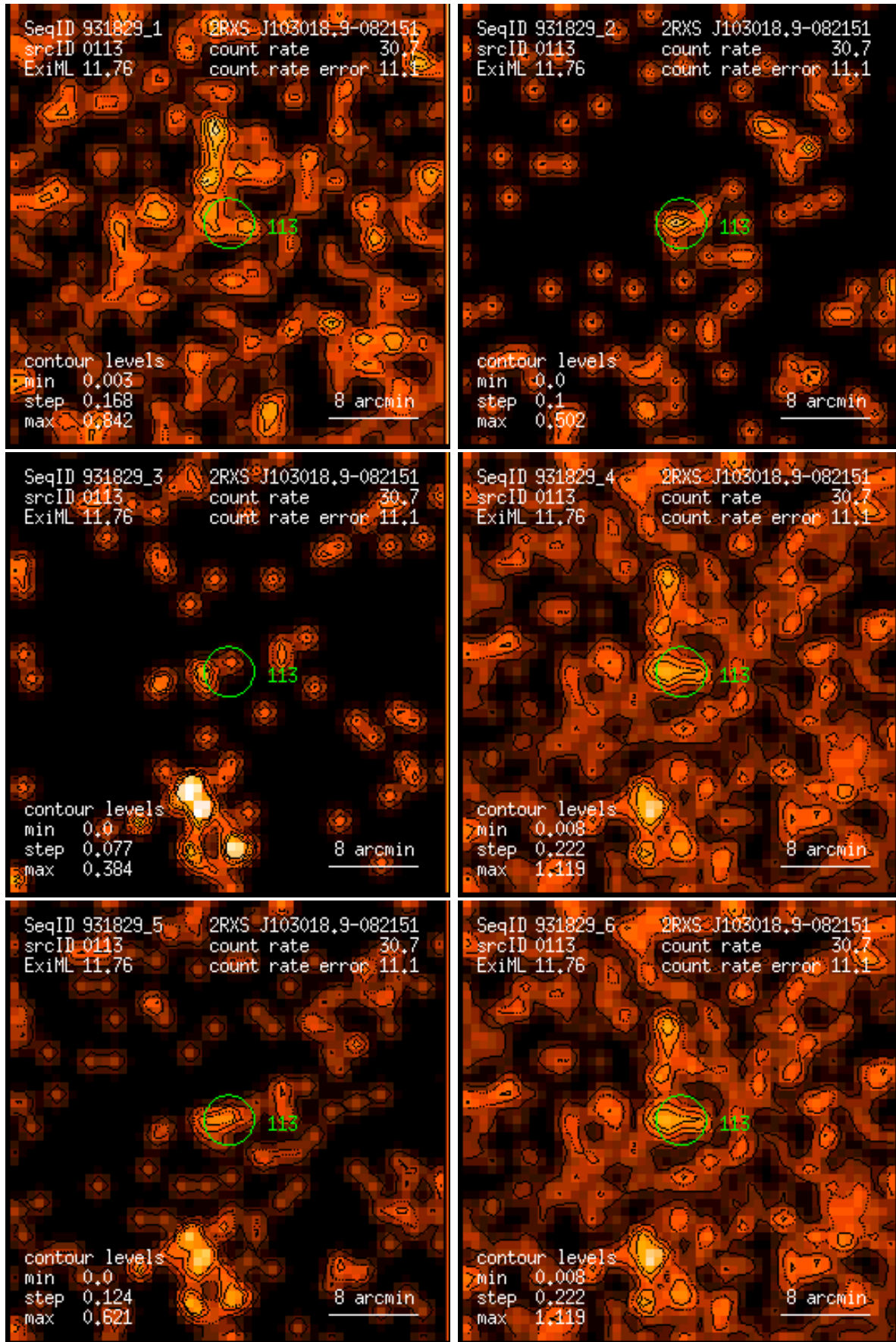
Figure 113: RASS 931829: detection 0113: band rate images, Gaussian filter: (1) PSPC channels 11 – 41, (2) 52 – 90, (3) 91 – 201, (4) 11 – 235, (5) 52 – 201, (6) 11 – 201. Broad band rates in counts/ks. Band rate contour levels in counts/ks/arcmin 2 .
