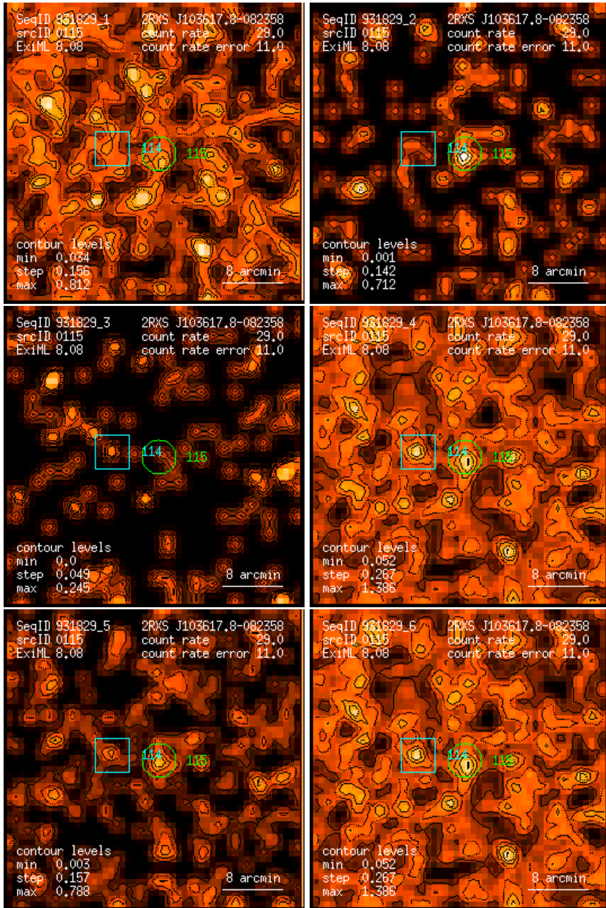
Figure 115: RASS 931829: detection 0115: band rate images, Gaussian filter: (1) PSPC channels 11 – 41, (2) 52 – 90, (3) 91 – 201, (4) 11 – 235, (5) 52 – 201, (6) 11 – 201. Broad band rates in counts/ks. Band rate contour levels in counts/ks/arcmin 2 .
