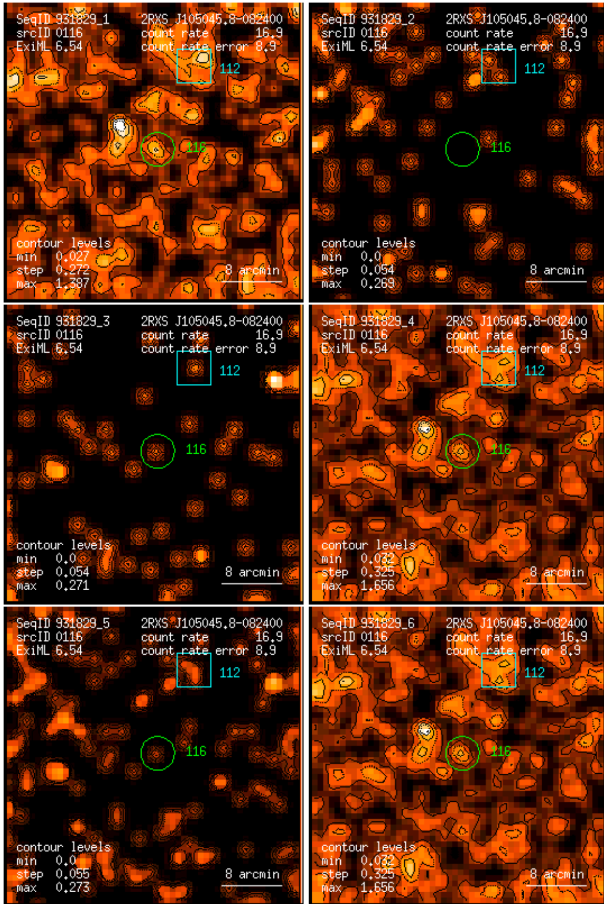
Figure 116: RASS 931829: detection 0116: band rate images, Gaussian filter: (1) PSPC channels 11 – 41, (2) 52 – 90, (3) 91 – 201, (4) 11 – 235, (5) 52 – 201, (6) 11 – 201. Broad band rates in counts/ks. Band rate contour levels in counts/ks/arcmin 2 .
