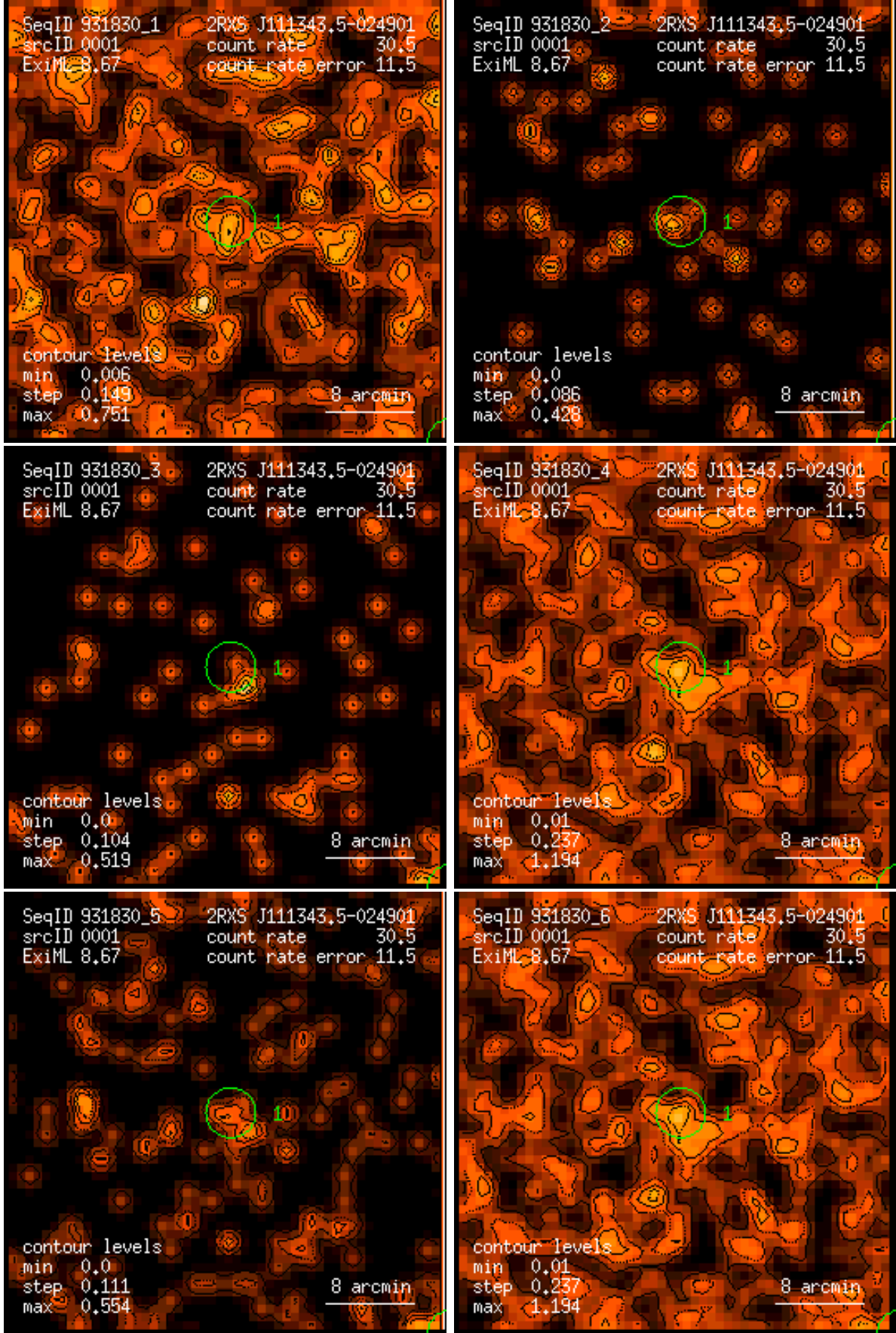
Figure 1: RASS 931830: detection 0001: band rate images, Gaussian filter: (1) PSPC channels 11 – 41, (2) 52 – 90, (3) 91 – 201, (4) 11 – 235, (5) 52 – 201, (6) 11 – 201. Broad band rates in counts/ks. Band rate contour levels in counts/ks/arcmin 2 .
