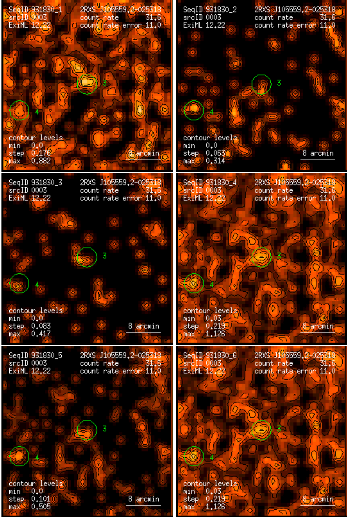
Figure 3: RASS 931830: detection 0003: band rate images, Gaussian filter: (1) PSPC channels 11 – 41, (2) 52 – 90, (3) 91 – 201, (4) 11 – 235, (5) 52 – 201, (6) 11 – 201. Broad band rates in counts/ks. Band rate contour levels in counts/ks/arcmin 2 .
