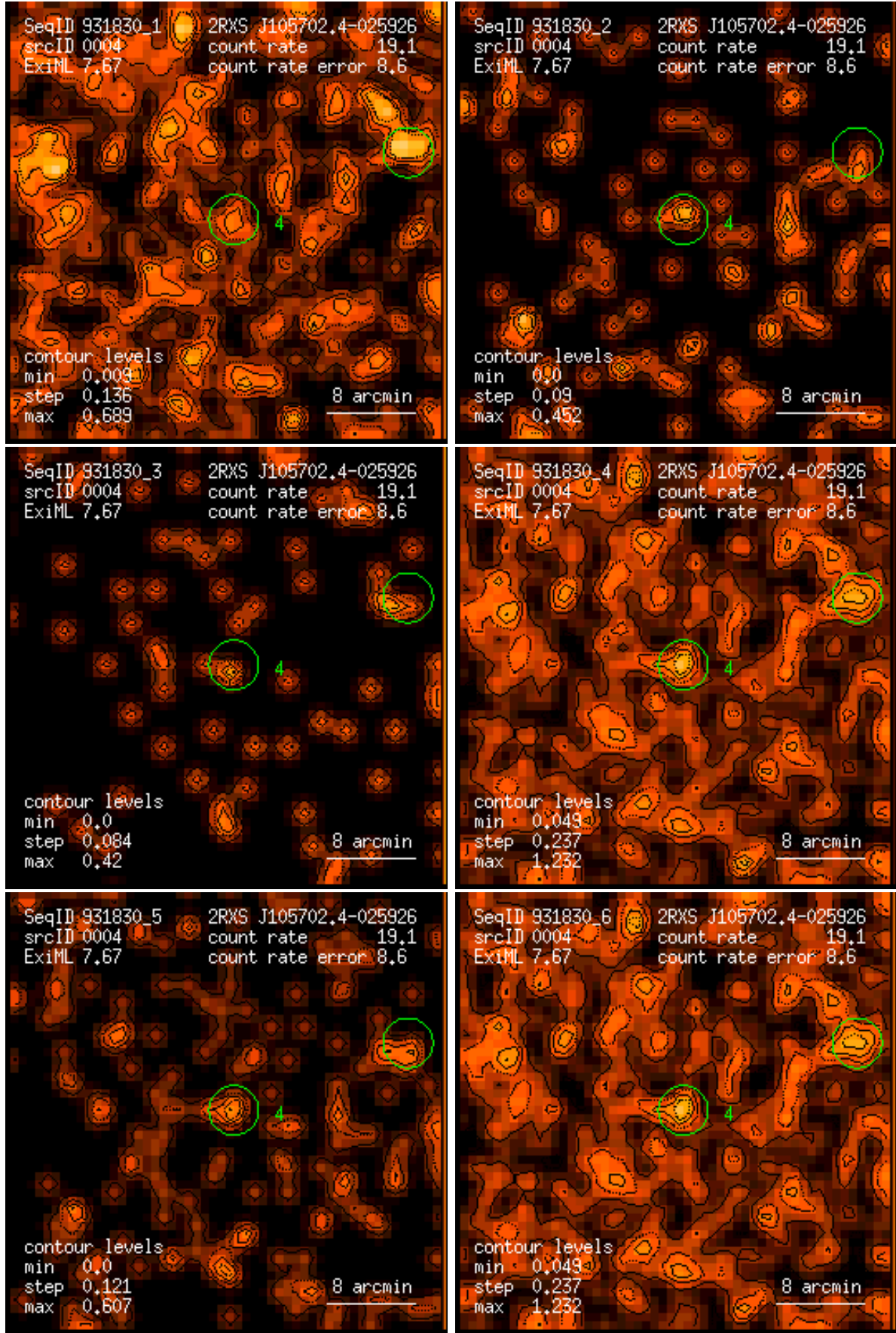
Figure 4: RASS 931830: detection 0004: band rate images, Gaussian filter: (1) PSPC channels 11 – 41, (2) 52 – 90, (3) 91 – 201, (4) 11 – 235, (5) 52 – 201, (6) 11 – 201. Broad band rates in counts/ks. Band rate contour levels in counts/ks/arcmin 2 .
