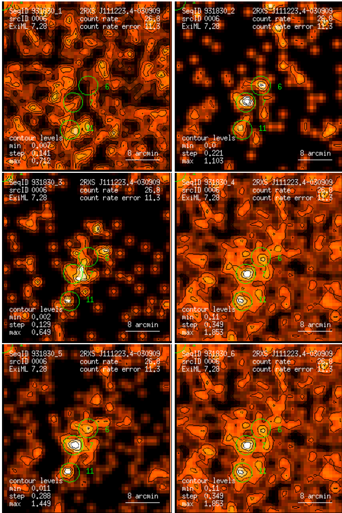
Figure 6: RASS 931830: detection 0006: band rate images, Gaussian filter: (1) PSPC channels 11 – 41, (2) 52 – 90, (3) 91 – 201, (4) 11 – 235, (5) 52 – 201, (6) 11 – 201. Broad band rates in counts/ks. Band rate contour levels in counts/ks/arcmin 2 .
