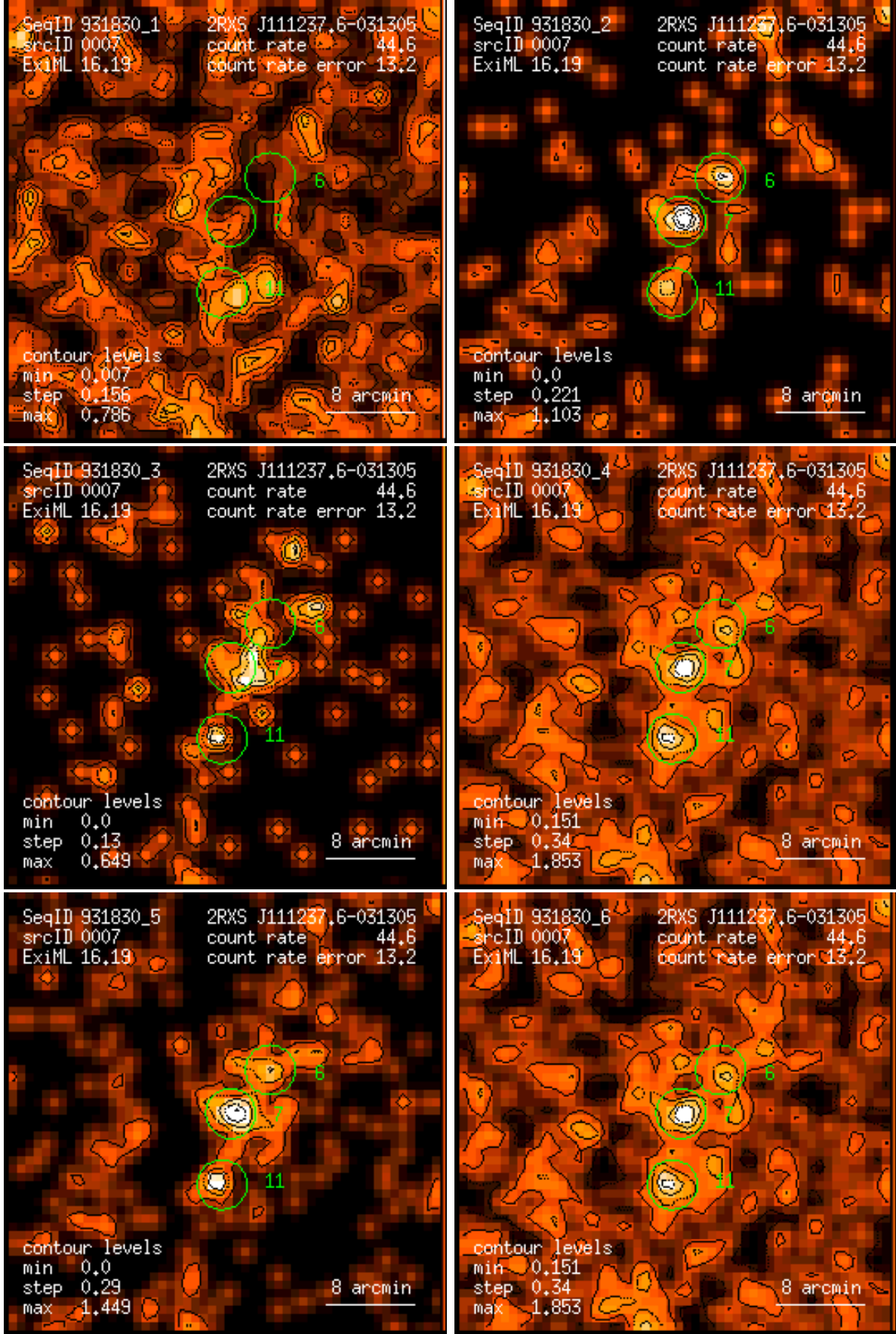
Figure 7: RASS 931830: detection 0007: band rate images, Gaussian filter: (1) PSPC channels 11 – 41, (2) 52 – 90, (3) 91 – 201, (4) 11 – 235, (5) 52 – 201, (6) 11 – 201. Broad band rates in counts/ks. Band rate contour levels in counts/ks/arcmin 2 .
