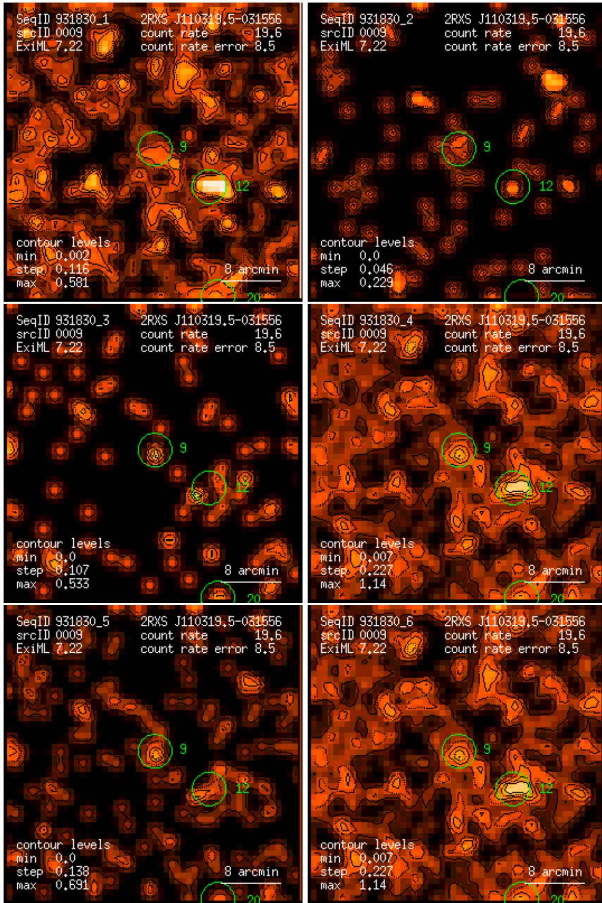
Figure 9: RASS 931830: detection 0009: band rate images, Gaussian filter: (1) PSPC channels 11 – 41, (2) 52 – 90, (3) 91 – 201, (4) 11 – 235, (5) 52 – 201, (6) 11 – 201. Broad band rates in counts/ks. Band rate contour levels in counts/ks/arcmin 2 .
