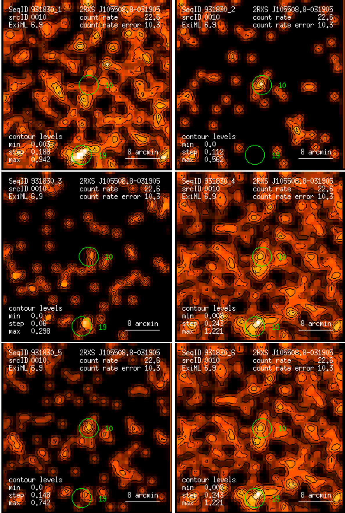
Figure 10: RASS 931830: detection 0010: band rate images, Gaussian filter: (1) PSPC channels 11 – 41, (2) 52 – 90, (3) 91 – 201, (4) 11 – 235, (5) 52 – 201, (6) 11 – 201. Broad band rates in counts/ks. Band rate contour levels in counts/ks/arcmin 2 .
