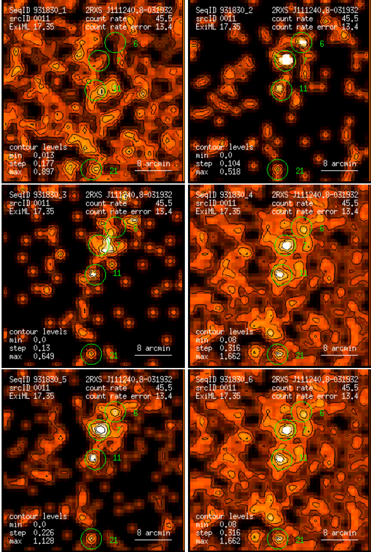
Figure 11: RASS 931830: detection 0011: band rate images, Gaussian filter: (1) PSPC channels 11 – 41, (2) 52 – 90, (3) 91 – 201, (4) 11 – 235, (5) 52 – 201, (6) 11 – 201. Broad band rates in counts/ks. Band rate contour levels in counts/ks/arcmin 2 .
