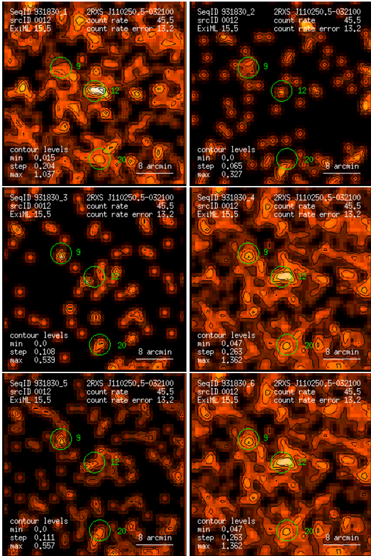
Figure 12: RASS 931830: detection 0012: band rate images, Gaussian filter: (1) PSPC channels 11 – 41, (2) 52 – 90, (3) 91 – 201, (4) 11 – 235, (5) 52 – 201, (6) 11 – 201. Broad band rates in counts/ks. Band rate contour levels in counts/ks/arcmin 2 .
