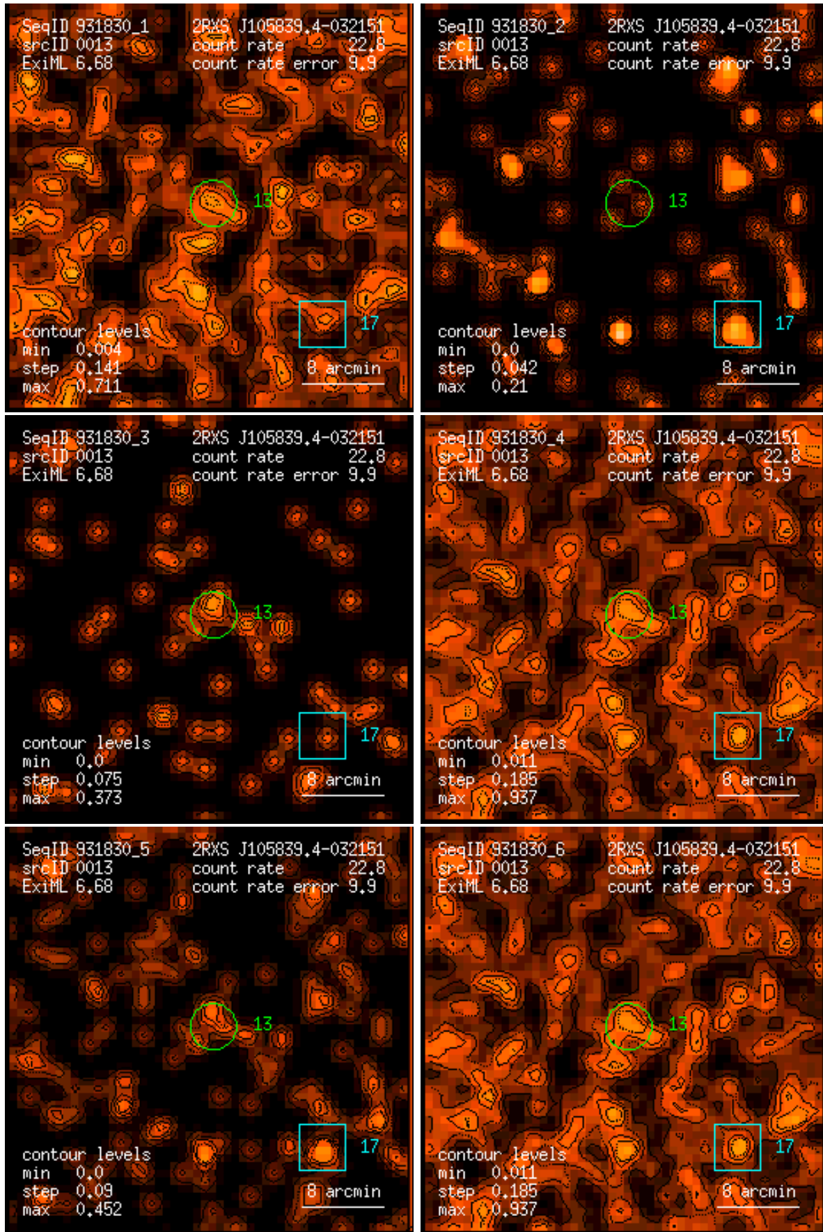
Figure 13: RASS 931830: detection 0013: band rate images, Gaussian filter: (1) PSPC channels 11 – 41, (2) 52 – 90, (3) 91 – 201, (4) 11 – 235, (5) 52 – 201, (6) 11 – 201. Broad band rates in counts/ks. Band rate contour levels in counts/ks/arcmin 2 .
