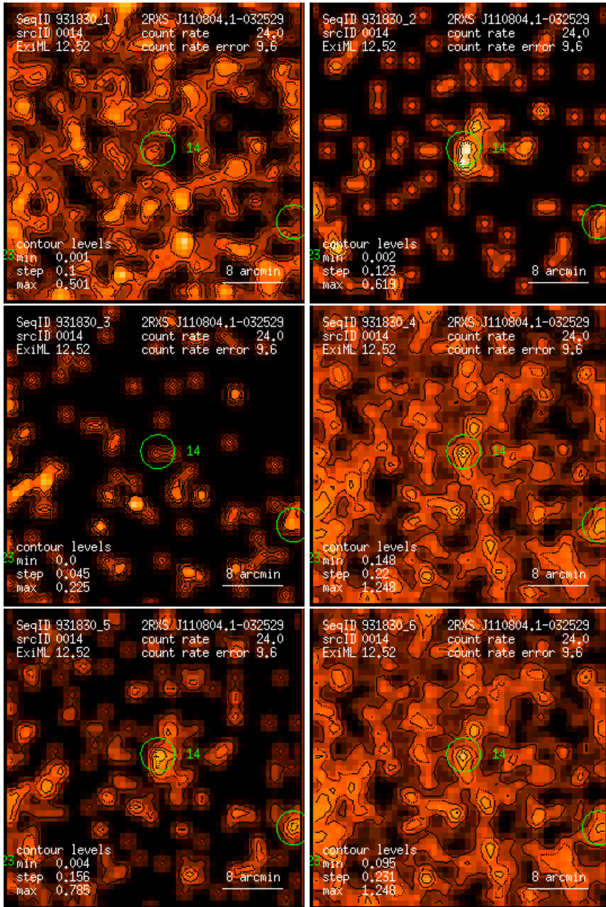
Figure 14: RASS 931830: detection 0014: band rate images, Gaussian filter: (1) PSPC channels 11 – 41, (2) 52 – 90, (3) 91 – 201, (4) 11 – 235, (5) 52 – 201, (6) 11 – 201. Broad band rates in counts/ks. Band rate contour levels in counts/ks/arcmin 2 .
