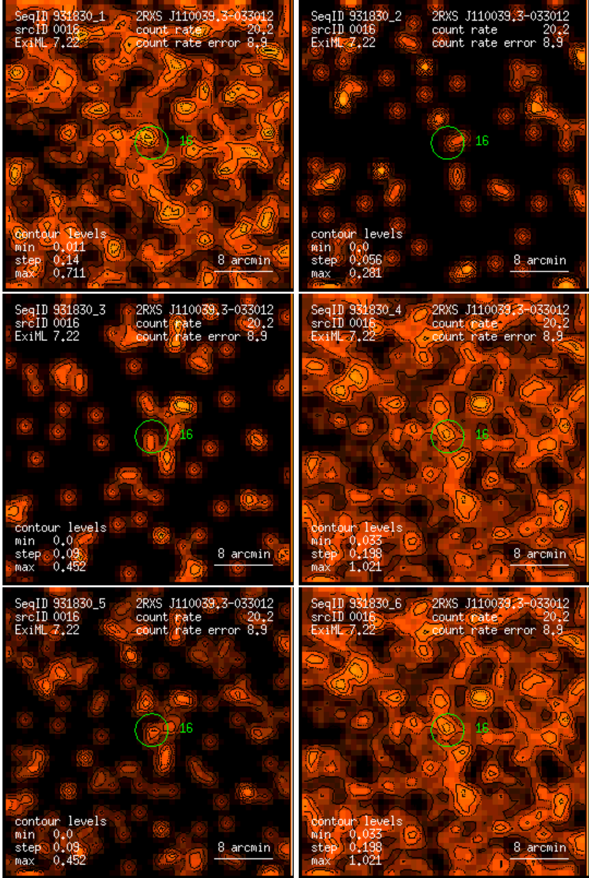
Figure 16: RASS 931830: detection 0016: band rate images, Gaussian filter: (1) PSPC channels 11 – 41, (2) 52 – 90, (3) 91 – 201, (4) 11 – 235, (5) 52 – 201, (6) 11 – 201. Broad band rates in counts/ks. Band rate contour levels in counts/ks/arcmin 2 .
