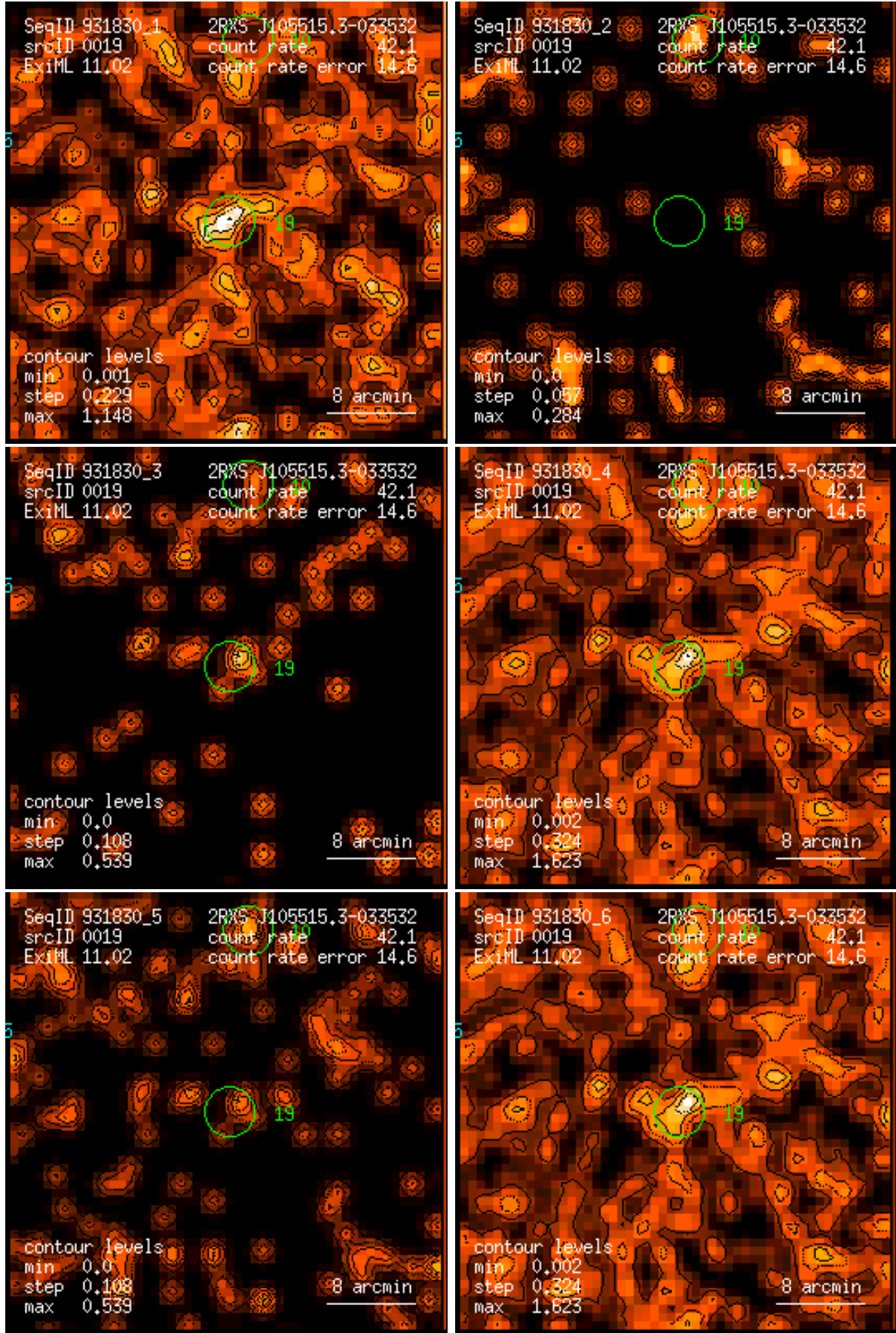
Figure 19: RASS 931830: detection 0019: band rate images, Gaussian filter: (1) PSPC channels 11 – 41, (2) 52 – 90, (3) 91 – 201, (4) 11 – 235, (5) 52 – 201, (6) 11 – 201. Broad band rates in counts/ks. Band rate contour levels in counts/ks/arcmin 2 .
