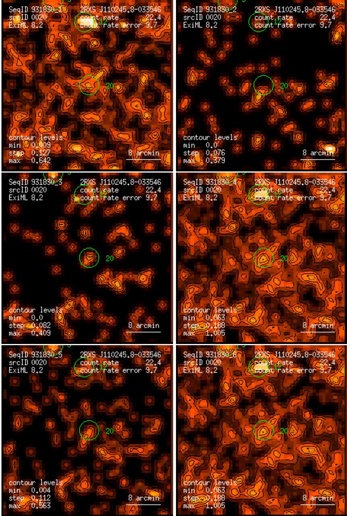
Figure 20: RASS 931830: detection 0020: band rate images, Gaussian filter: (1) PSPC channels 11 – 41, (2) 52 – 90, (3) 91 – 201, (4) 11 – 235, (5) 52 – 201, (6) 11 – 201. Broad band rates in counts/ks. Band rate contour levels in counts/ks/arcmin 2 .
