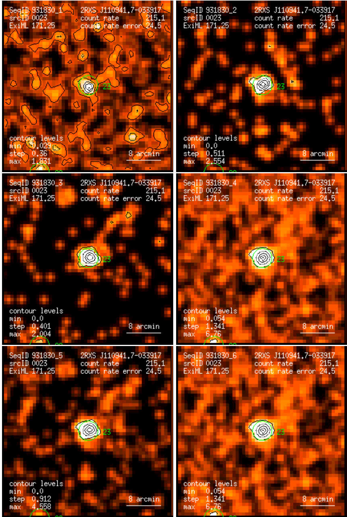
Figure 23: RASS 931830: detection 0023: band rate images, Gaussian filter: (1) PSPC channels 11 – 41, (2) 52 – 90, (3) 91 – 201, (4) 11 – 235, (5) 52 – 201, (6) 11 – 201. Broad band rates in counts/ks. Band rate contour levels in counts/ks/arcmin 2 .
