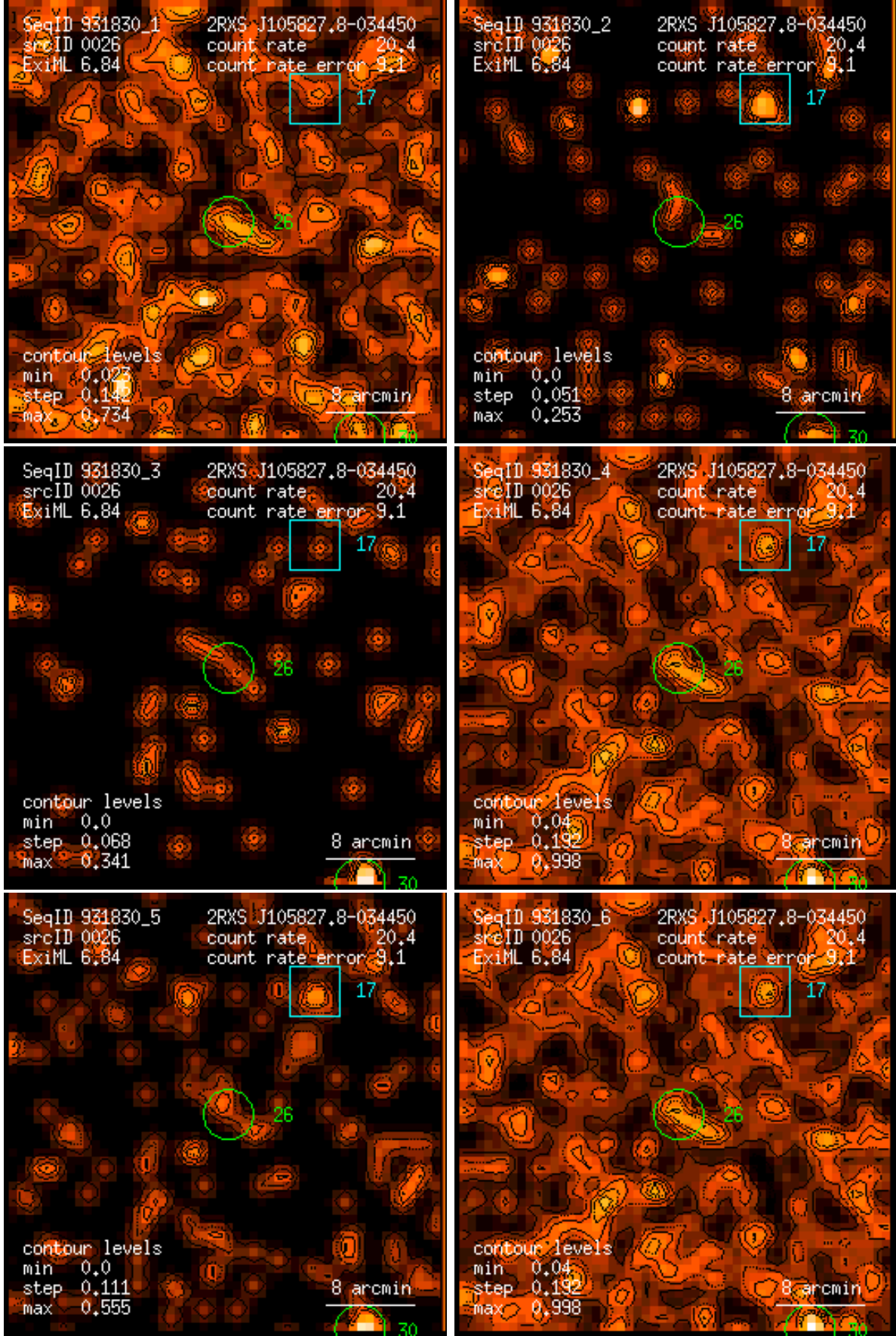
Figure 26: RASS 931830: detection 0026: band rate images, Gaussian filter: (1) PSPC channels 11 – 41, (2) 52 – 90, (3) 91 – 201, (4) 11 – 235, (5) 52 – 201, (6) 11 – 201. Broad band rates in counts/ks. Band rate contour levels in counts/ks/arcmin 2 .
