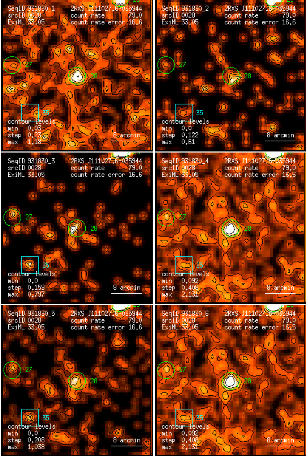
Figure 28: RASS 931830: detection 0028: band rate images, Gaussian filter: (1) PSPC channels 11 – 41, (2) 52 – 90, (3) 91 – 201, (4) 11 – 235, (5) 52 – 201, (6) 11 – 201. Broad band rates in counts/ks. Band rate contour levels in counts/ks/arcmin 2 .
