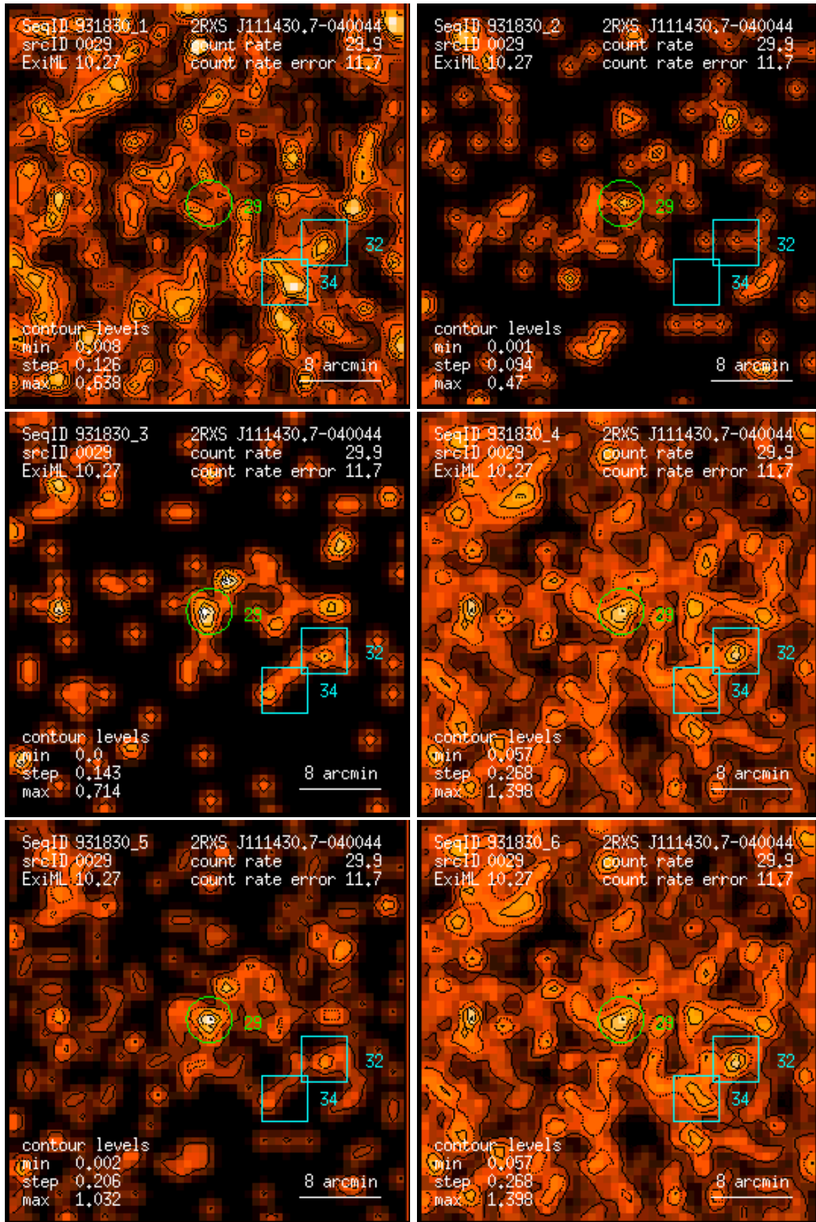
Figure 29: RASS 931830: detection 0029: band rate images, Gaussian filter: (1) PSPC channels 11 – 41, (2) 52 – 90, (3) 91 – 201, (4) 11 – 235, (5) 52 – 201, (6) 11 – 201. Broad band rates in counts/ks. Band rate contour levels in counts/ks/arcmin 2 .
