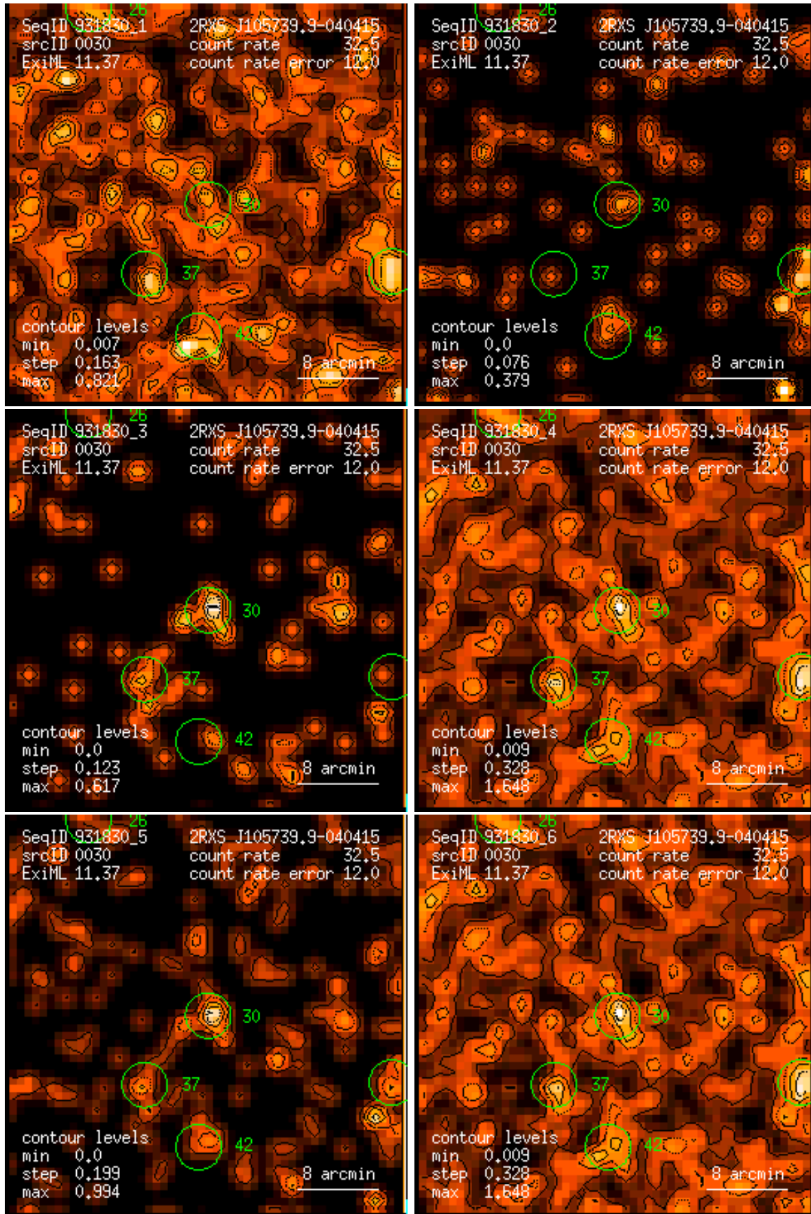
Figure 30: RASS 931830: detection 0030: band rate images, Gaussian filter: (1) PSPC channels 11 – 41, (2) 52 – 90, (3) 91 – 201, (4) 11 – 235, (5) 52 – 201, (6) 11 – 201. Broad band rates in counts/ks. Band rate contour levels in counts/ks/arcmin 2 .
