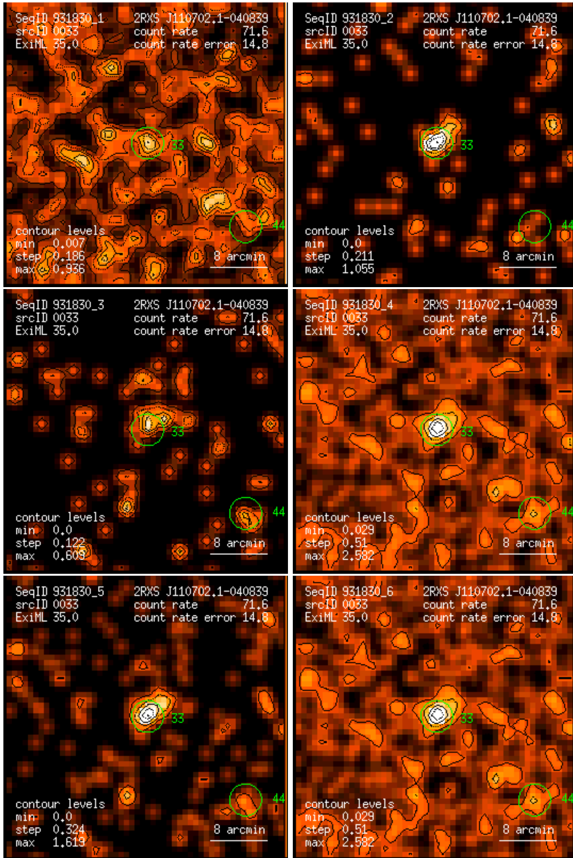
Figure 33: RASS 931830: detection 0033: band rate images, Gaussian filter: (1) PSPC channels 11 – 41, (2) 52 – 90, (3) 91 – 201, (4) 11 – 235, (5) 52 – 201, (6) 11 – 201. Broad band rates in counts/ks. Band rate contour levels in counts/ks/arcmin 2 .
