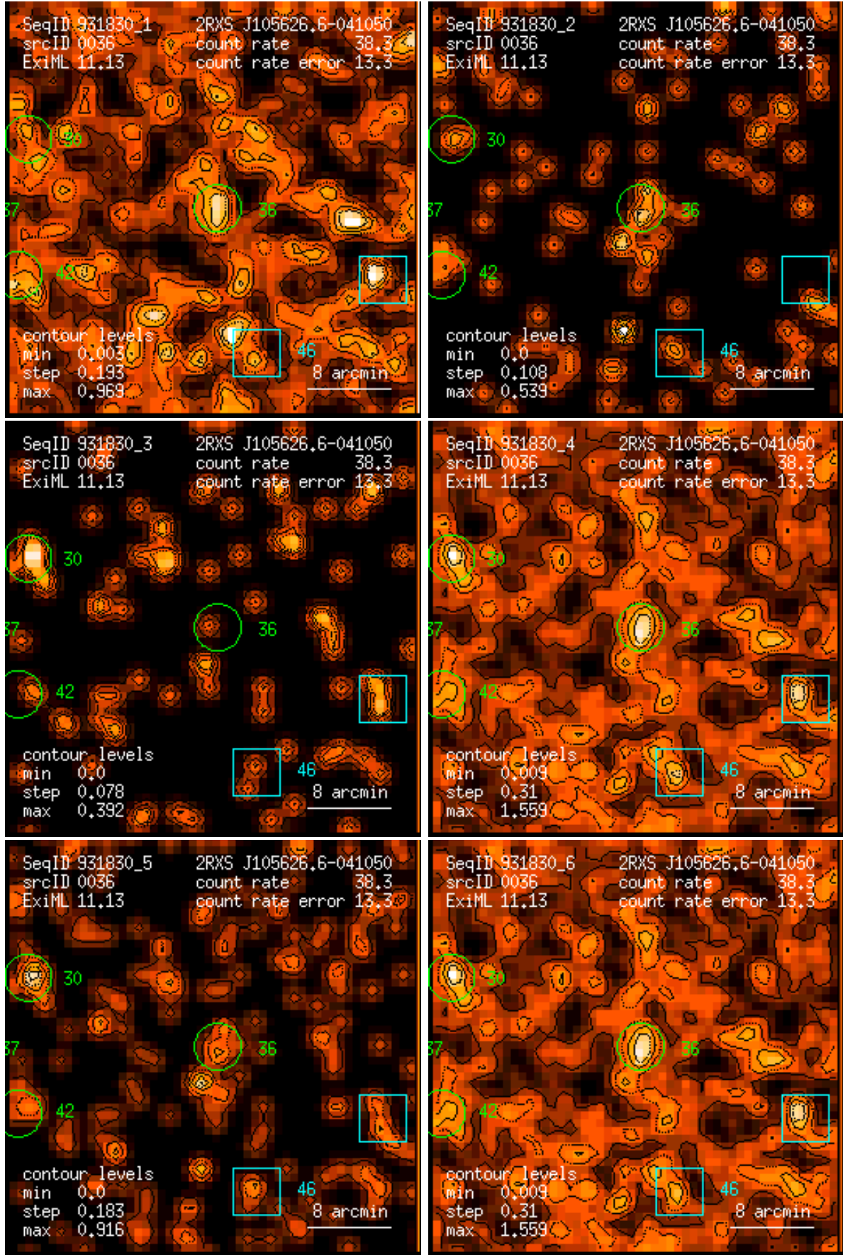
Figure 36: RASS 931830: detection 0036: band rate images, Gaussian filter: (1) PSPC channels 11 – 41, (2) 52 – 90, (3) 91 – 201, (4) 11 – 235, (5) 52 – 201, (6) 11 – 201. Broad band rates in counts/ks. Band rate contour levels in counts/ks/arcmin 2 .
