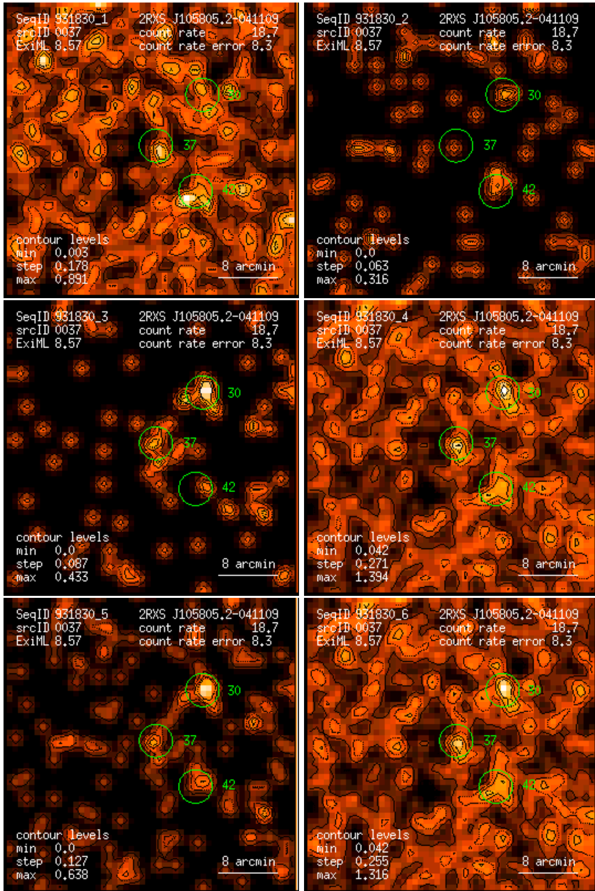
Figure 37: RASS 931830: detection 0037: band rate images, Gaussian filter: (1) PSPC channels 11 – 41, (2) 52 – 90, (3) 91 – 201, (4) 11 – 235, (5) 52 – 201, (6) 11 – 201. Broad band rates in counts/ks. Band rate contour levels in counts/ks/arcmin 2 .
