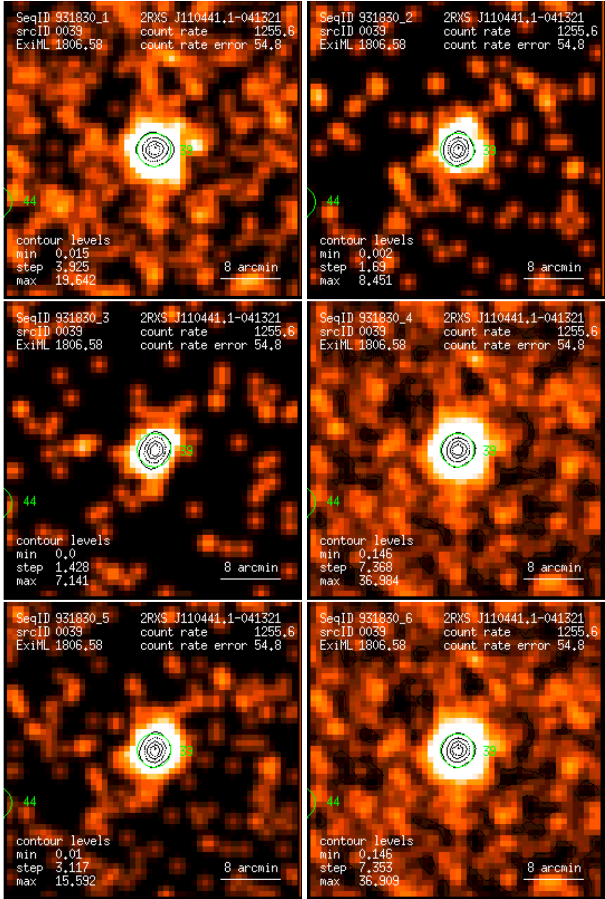
Figure 39: RASS 931830: detection 0039: band rate images, Gaussian filter: (1) PSPC channels 11 – 41, (2) 52 – 90, (3) 91 – 201, (4) 11 – 235, (5) 52 – 201, (6) 11 – 201. Broad band rates in counts/ks. Band rate contour levels in counts/ks/arcmin 2 .
