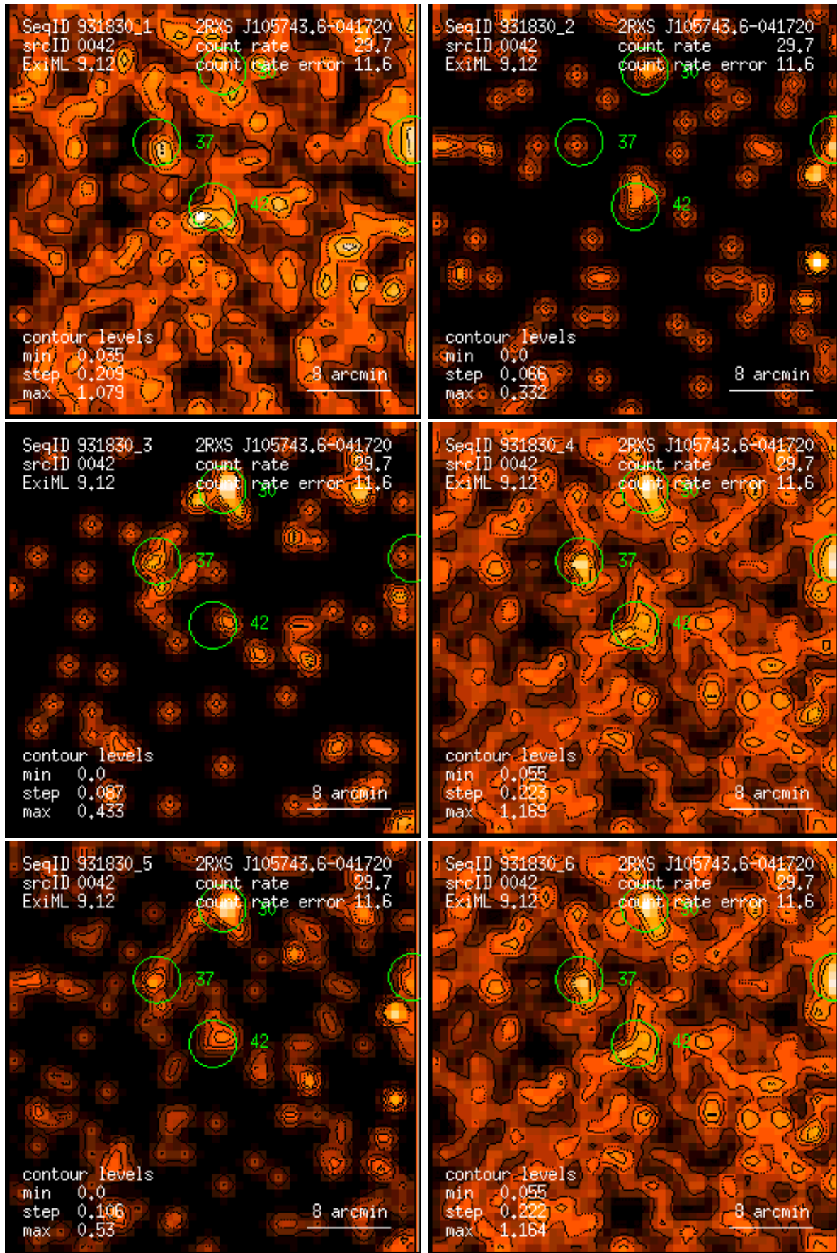
Figure 42: RASS 931830: detection 0042: band rate images, Gaussian filter: (1) PSPC channels 11 – 41, (2) 52 – 90, (3) 91 – 201, (4) 11 – 235, (5) 52 – 201, (6) 11 – 201. Broad band rates in counts/ks. Band rate contour levels in counts/ks/arcmin 2 .
