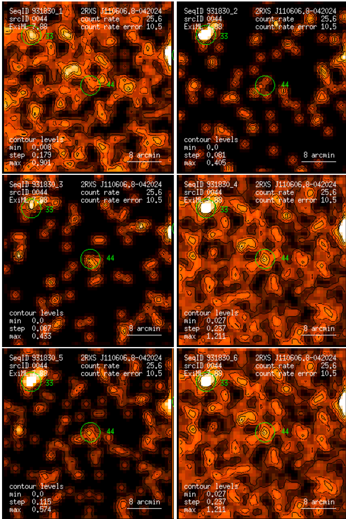
Figure 44: RASS 931830: detection 0044: band rate images, Gaussian filter: (1) PSPC channels 11 – 41, (2) 52 – 90, (3) 91 – 201, (4) 11 – 235, (5) 52 – 201, (6) 11 – 201. Broad band rates in counts/ks. Band rate contour levels in counts/ks/arcmin 2 .
