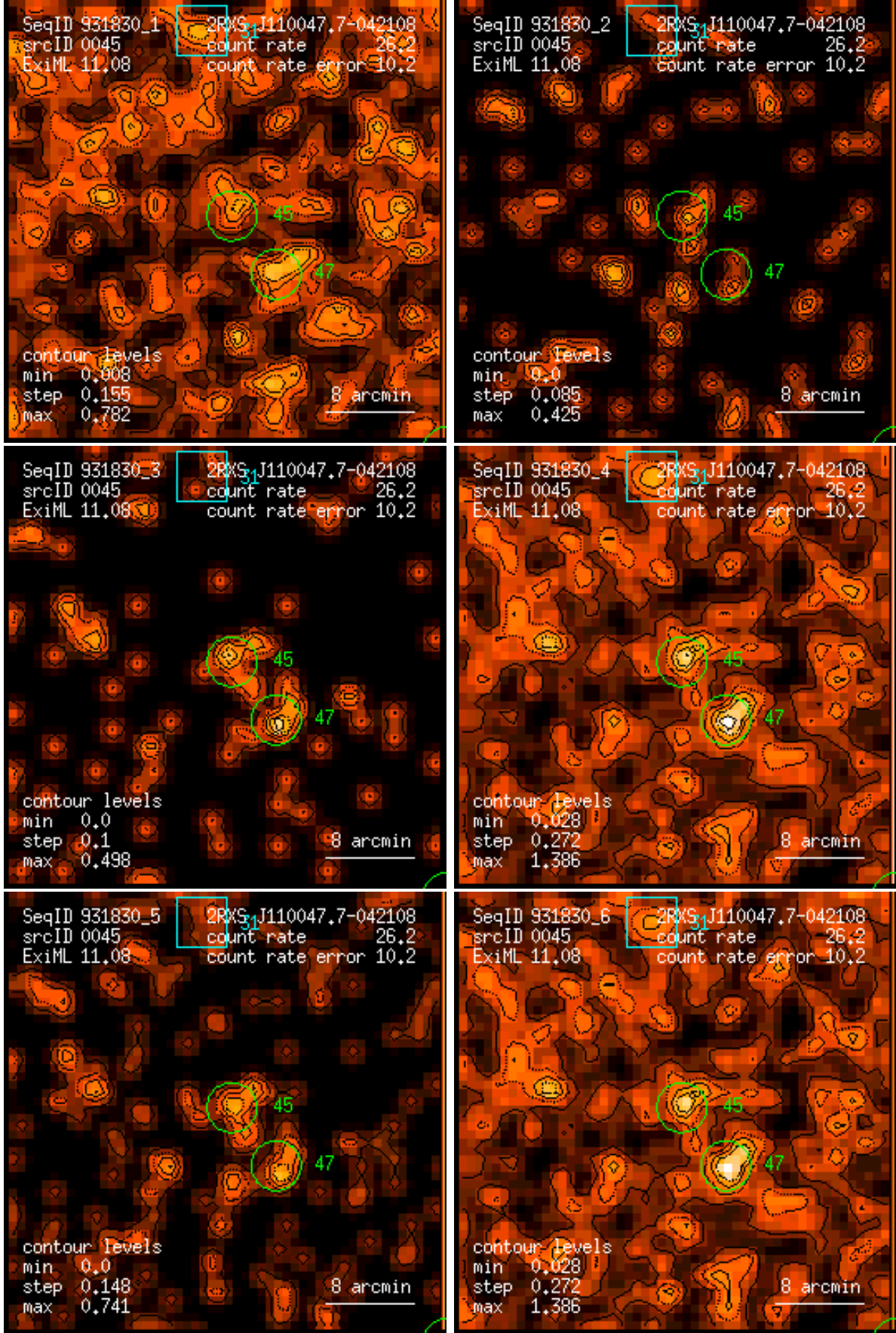
Figure 45: RASS 931830: detection 0045: band rate images, Gaussian filter: (1) PSPC channels 11 – 41, (2) 52 – 90, (3) 91 – 201, (4) 11 – 235, (5) 52 – 201, (6) 11 – 201. Broad band rates in counts/ks. Band rate contour levels in counts/ks/arcmin 2 .
