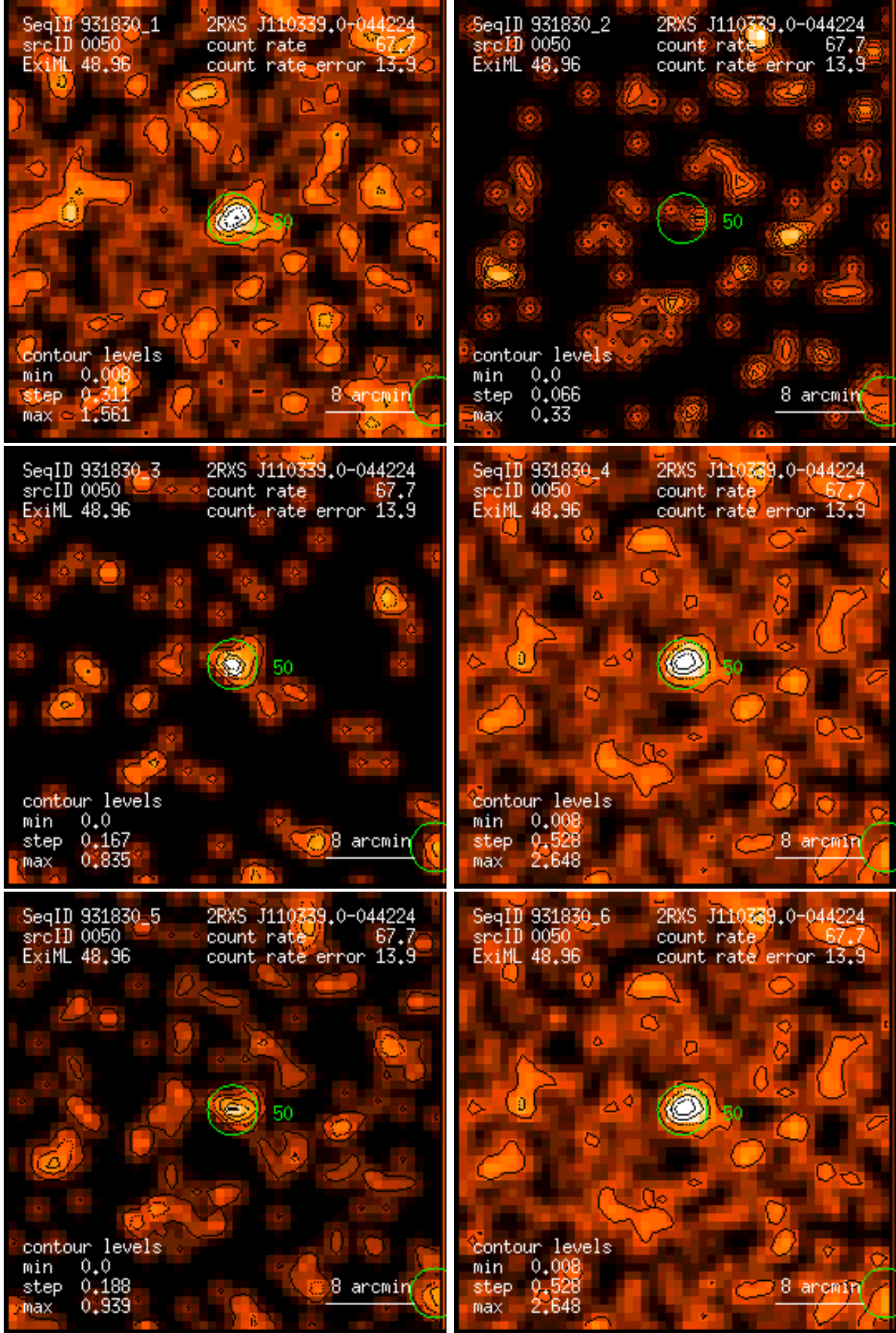
Figure 50: RASS 931830: detection 0050: band rate images, Gaussian filter: (1) PSPC channels 11 – 41, (2) 52 – 90, (3) 91 – 201, (4) 11 – 235, (5) 52 – 201, (6) 11 – 201. Broad band rates in counts/ks. Band rate contour levels in counts/ks/arcmin 2 .
