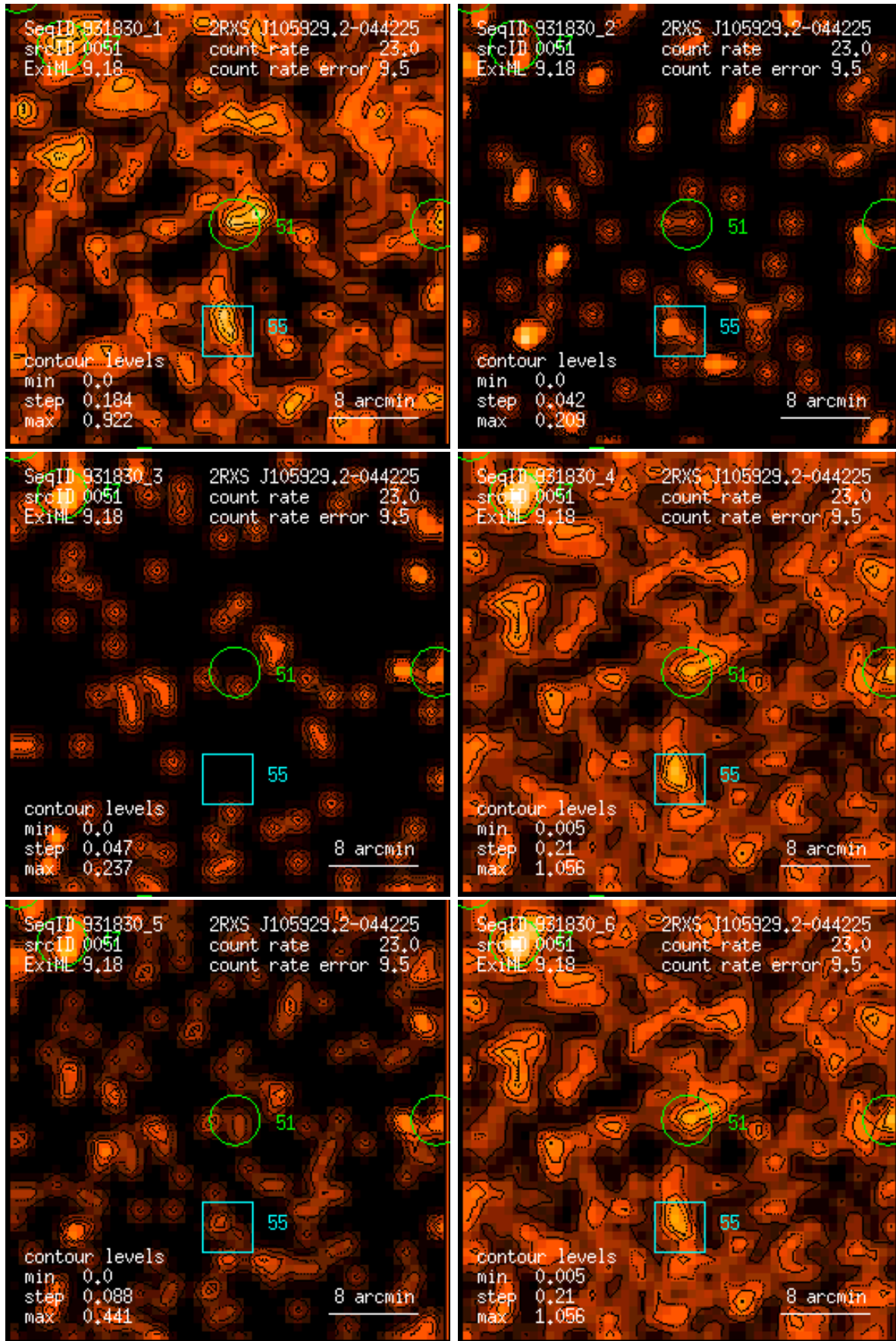
Figure 51: RASS 931830: detection 0051: band rate images, Gaussian filter: (1) PSPC channels 11 – 41, (2) 52 – 90, (3) 91 – 201, (4) 11 – 235, (5) 52 – 201, (6) 11 – 201. Broad band rates in counts/ks. Band rate contour levels in counts/ks/arcmin 2 .
