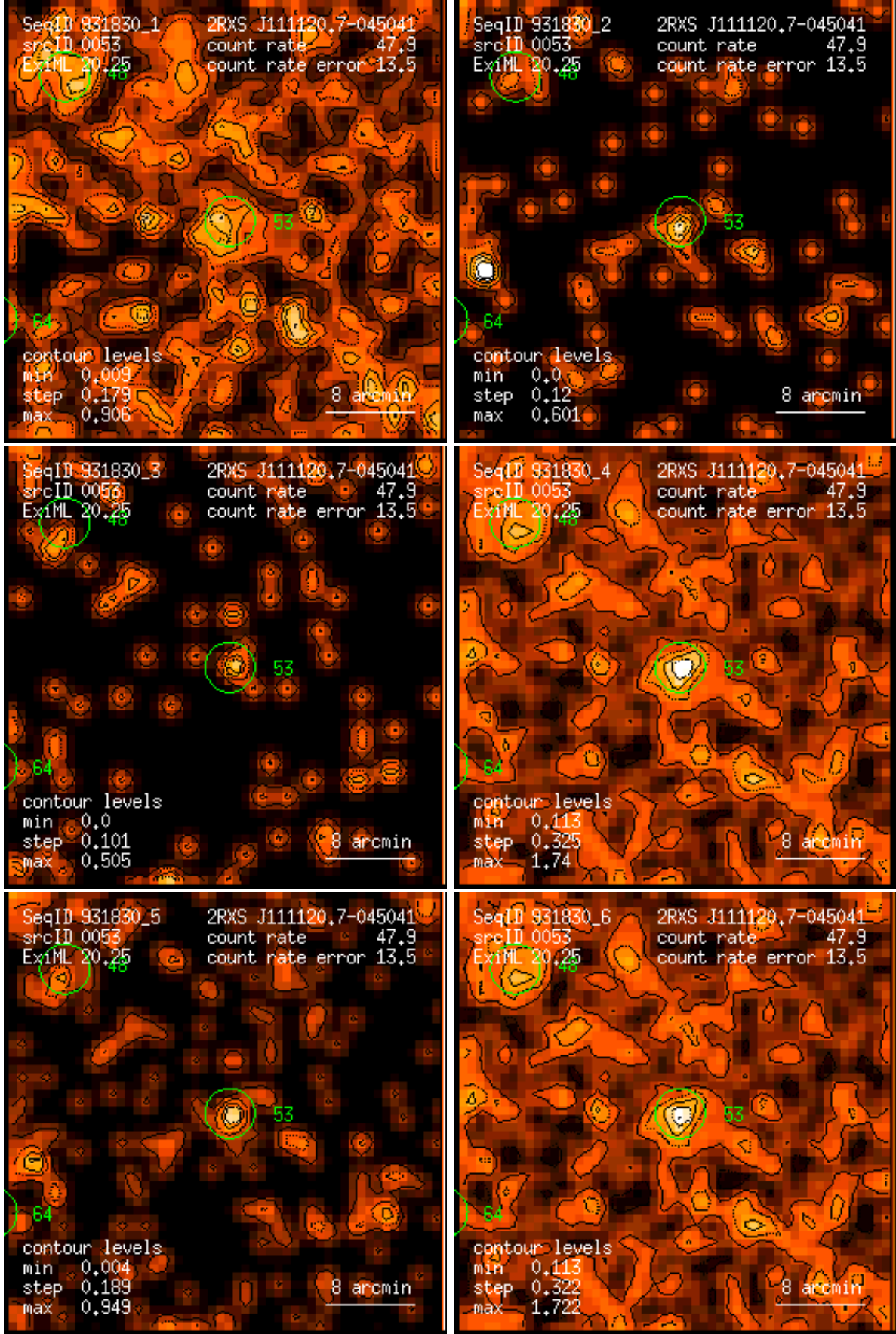
Figure 53: RASS 931830: detection 0053: band rate images, Gaussian filter: (1) PSPC channels 11 – 41, (2) 52 – 90, (3) 91 – 201, (4) 11 – 235, (5) 52 – 201, (6) 11 – 201. Broad band rates in counts/ks. Band rate contour levels in counts/ks/arcmin 2 .
