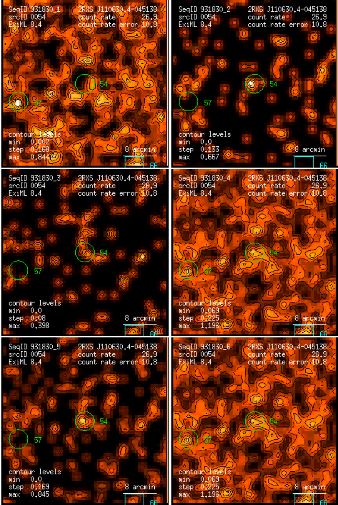
Figure 54: RASS 931830: detection 0054: band rate images, Gaussian filter: (1) PSPC channels 11 – 41, (2) 52 – 90, (3) 91 – 201, (4) 11 – 235, (5) 52 – 201, (6) 11 – 201. Broad band rates in counts/ks. Band rate contour levels in counts/ks/arcmin 2 .
