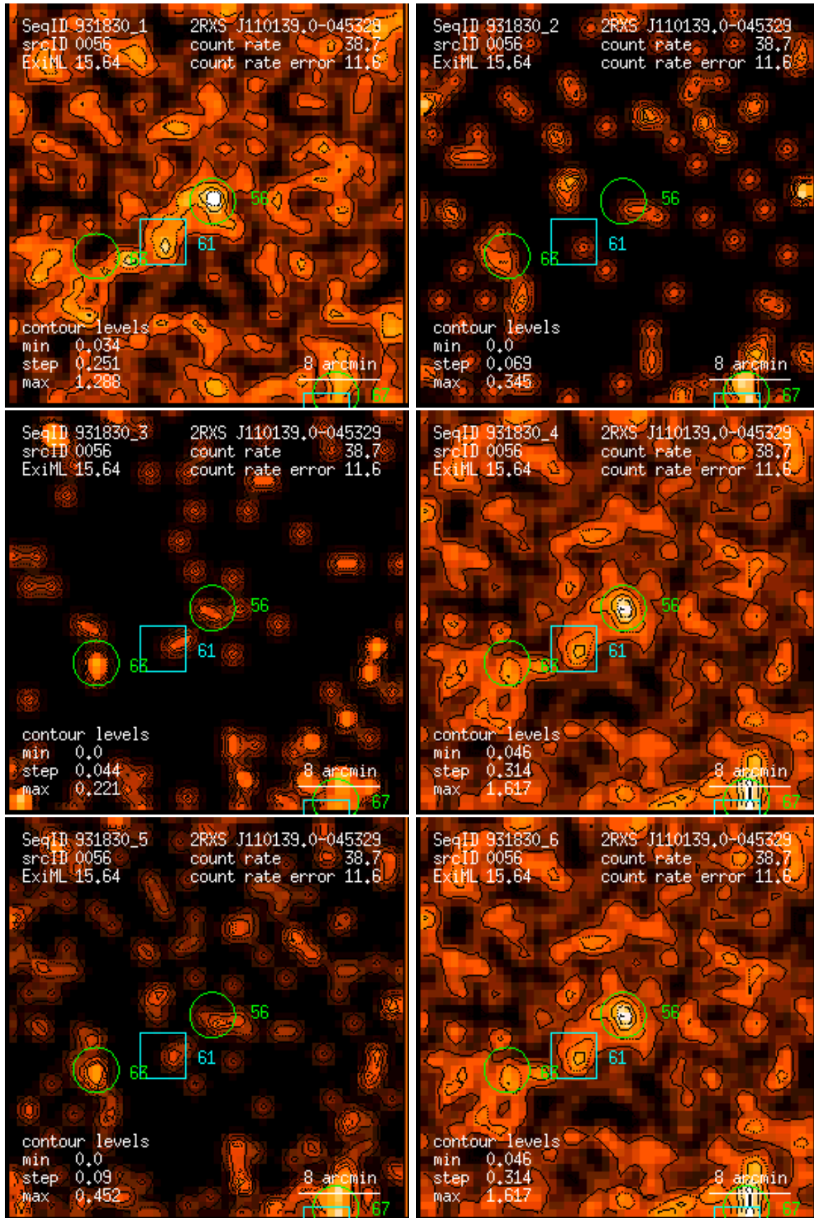
Figure 56: RASS 931830: detection 0056: band rate images, Gaussian filter: (1) PSPC channels 11 – 41, (2) 52 – 90, (3) 91 – 201, (4) 11 – 235, (5) 52 – 201, (6) 11 – 201. Broad band rates in counts/ks. Band rate contour levels in counts/ks/arcmin 2 .
