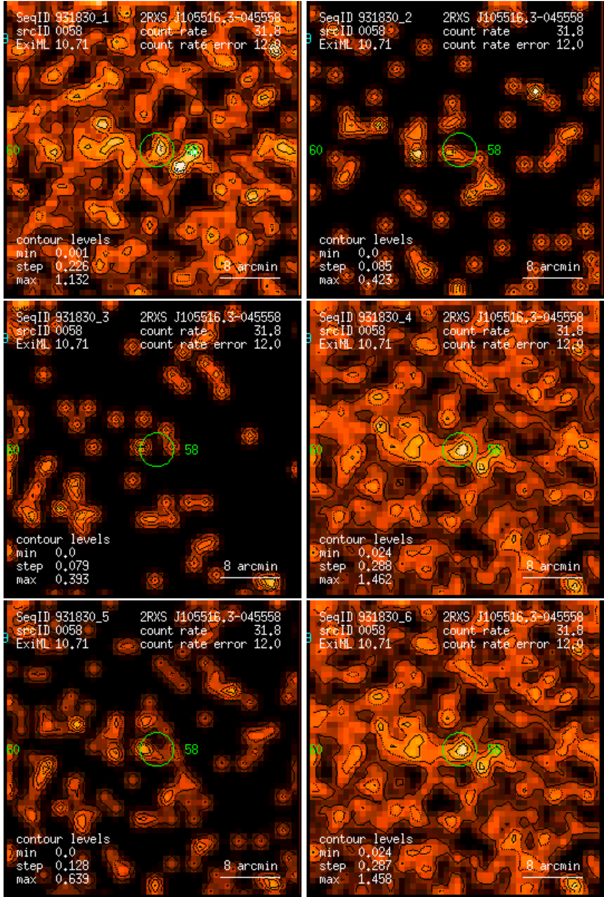
Figure 58: RASS 931830: detection 0058: band rate images, Gaussian filter: (1) PSPC channels 11 – 41, (2) 52 – 90, (3) 91 – 201, (4) 11 – 235, (5) 52 – 201, (6) 11 – 201. Broad band rates in counts/ks. Band rate contour levels in counts/ks/arcmin 2 .
