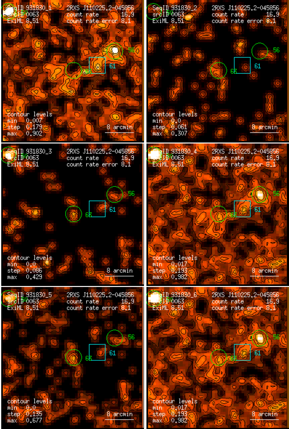
Figure 63: RASS 931830: detection 0063: band rate images, Gaussian filter: (1) PSPC channels 11 – 41, (2) 52 – 90, (3) 91 – 201, (4) 11 – 235, (5) 52 – 201, (6) 11 – 201. Broad band rates in counts/ks. Band rate contour levels in counts/ks/arcmin 2 .
