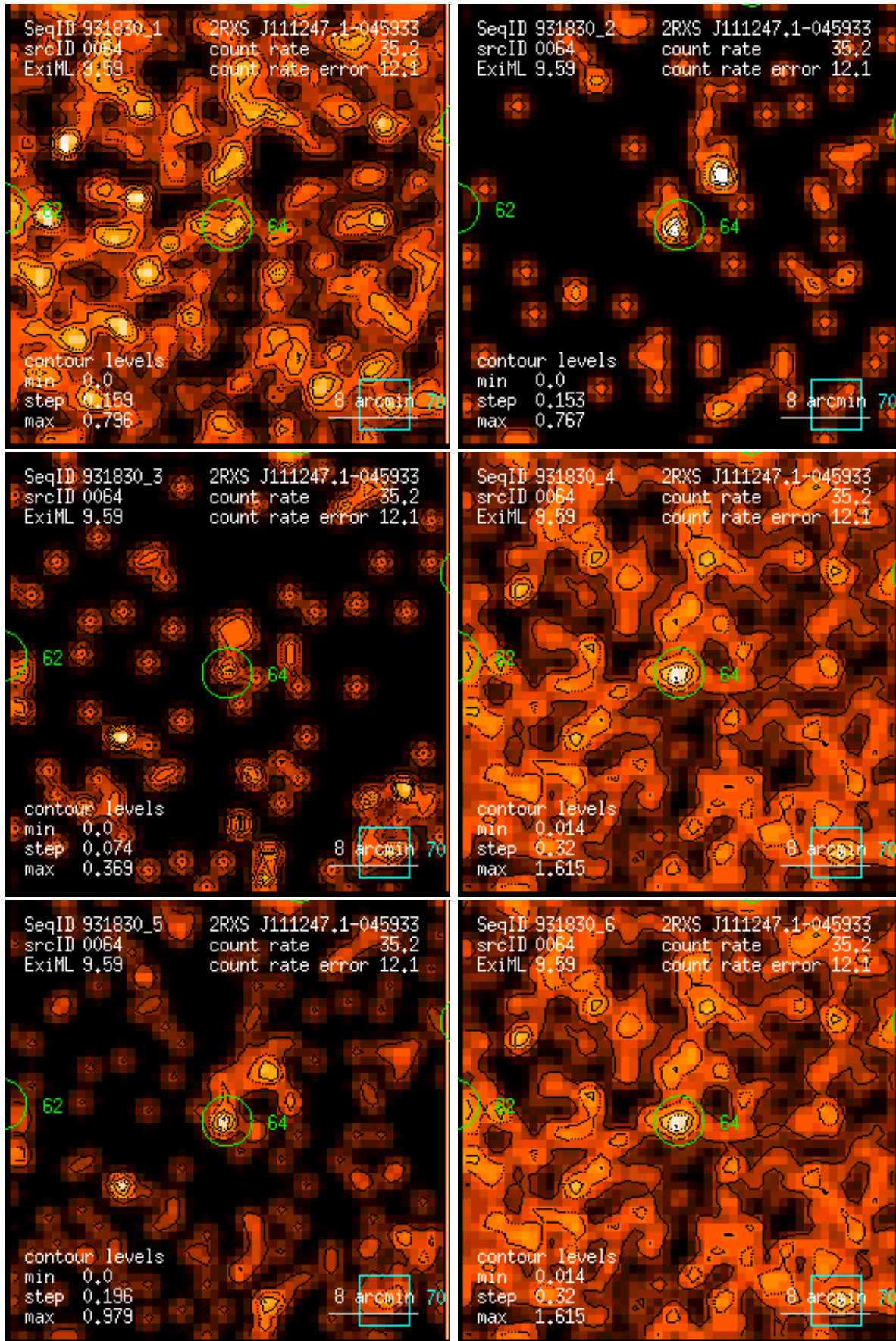
Figure 64: RASS 931830: detection 0064: band rate images, Gaussian filter: (1) PSPC channels 11 – 41, (2) 52 – 90, (3) 91 – 201, (4) 11 – 235, (5) 52 – 201, (6) 11 – 201. Broad band rates in counts/ks. Band rate contour levels in counts/ks/arcmin 2 .
