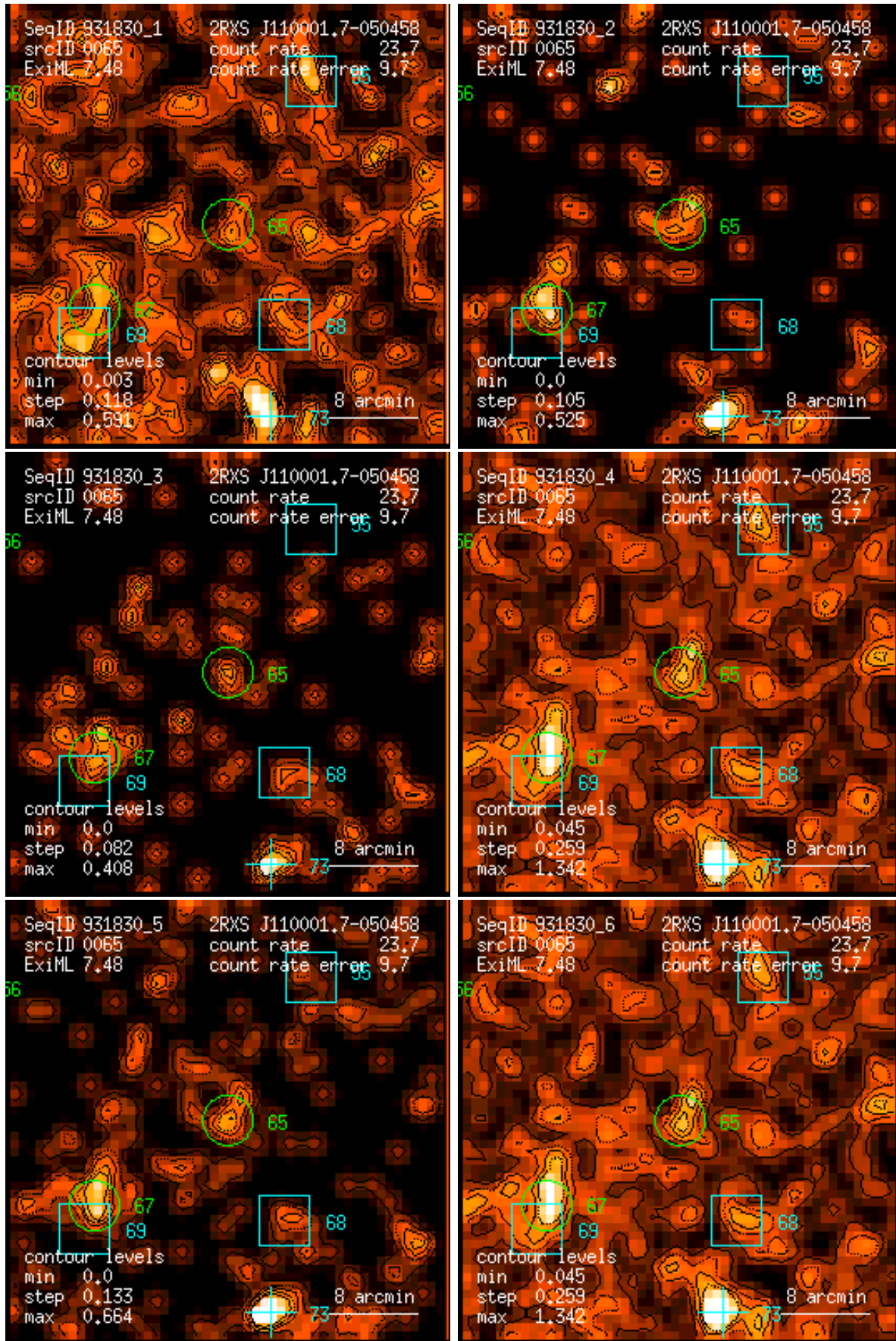
Figure 65: RASS 931830: detection 0065: band rate images, Gaussian filter: (1) PSPC channels 11 – 41, (2) 52 – 90, (3) 91 – 201, (4) 11 – 235, (5) 52 – 201, (6) 11 – 201. Broad band rates in counts/ks. Band rate contour levels in counts/ks/arcmin 2 .
