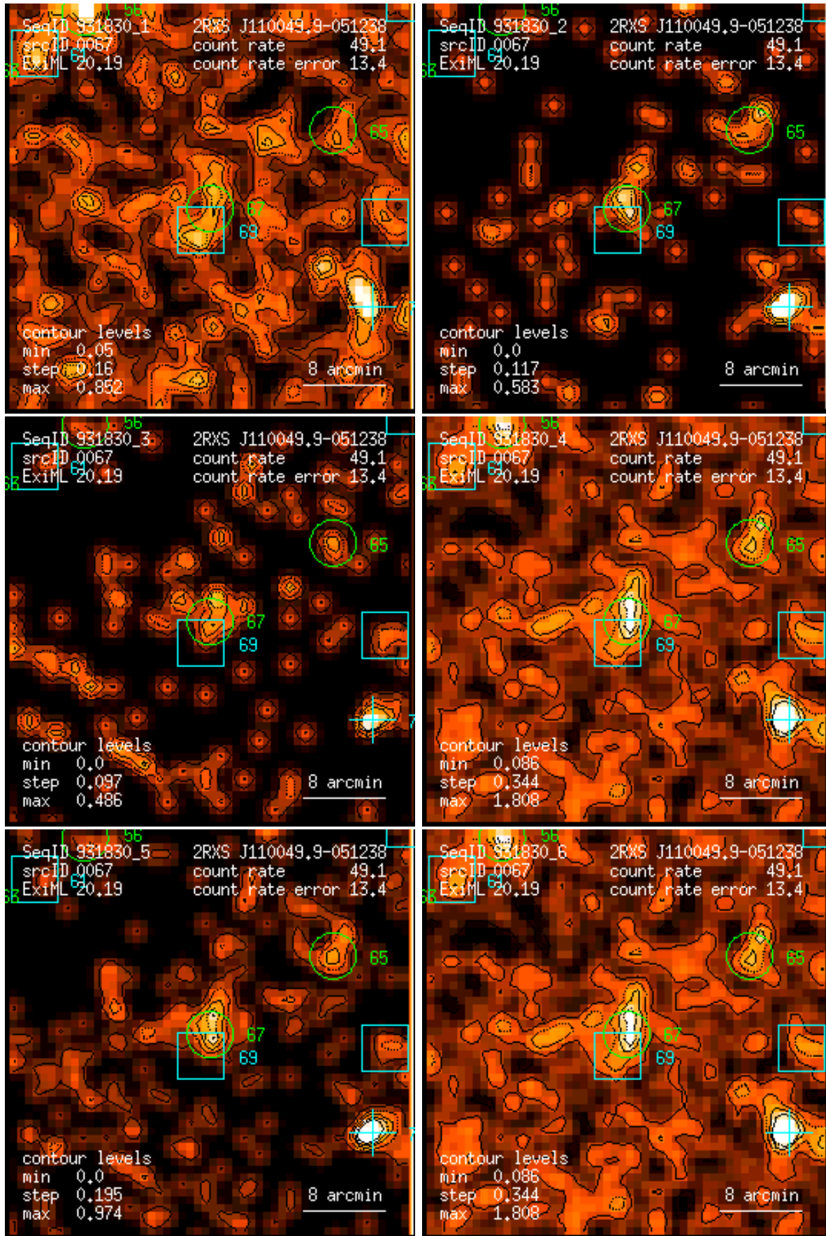
Figure 67: RASS 931830: detection 0067: band rate images, Gaussian filter: (1) PSPC channels 11 – 41, (2) 52 – 90, (3) 91 – 201, (4) 11 – 235, (5) 52 – 201, (6) 11 – 201. Broad band rates in counts/ks. Band rate contour levels in counts/ks/arcmin 2 .
