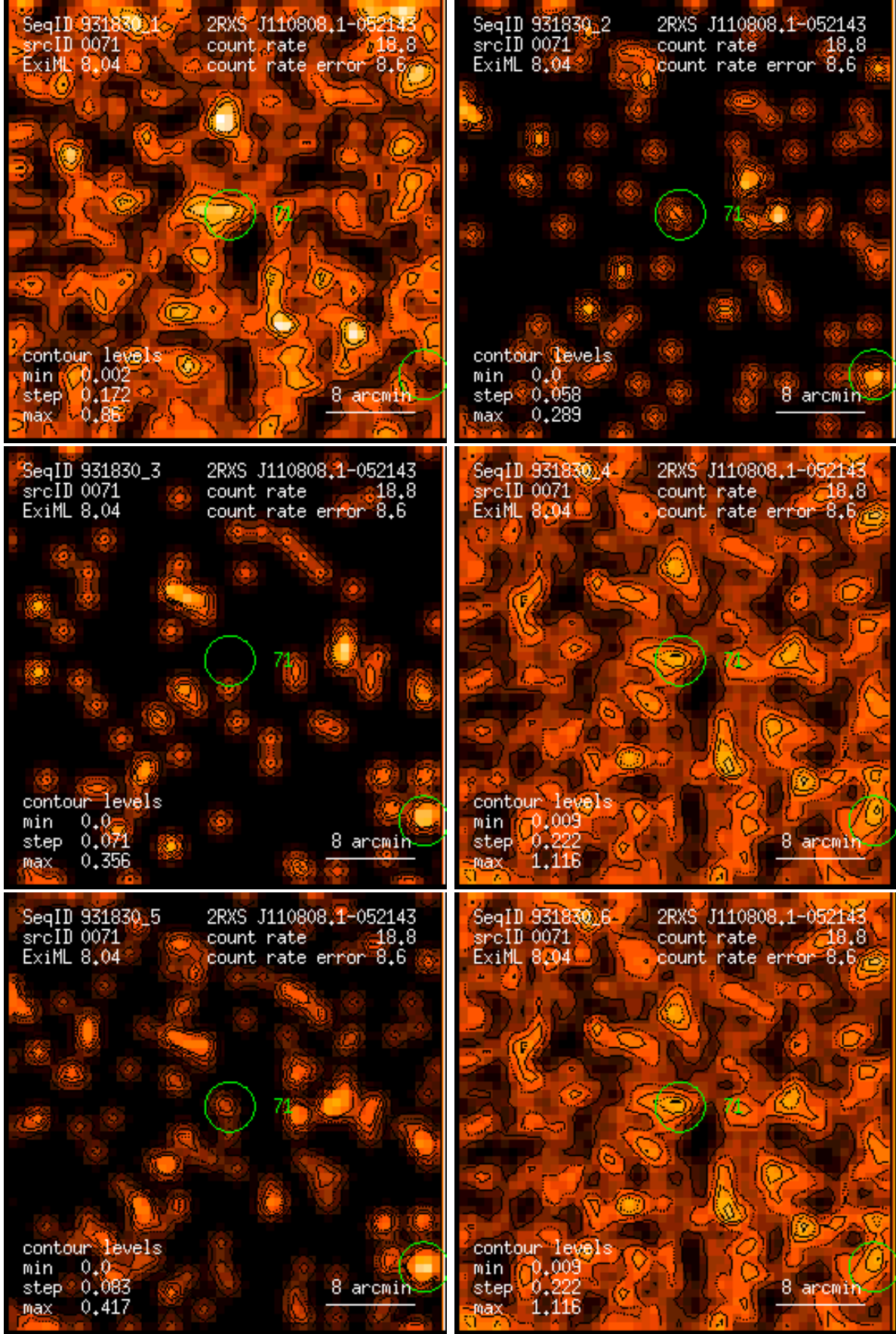
Figure 71: RASS 931830: detection 0071: band rate images, Gaussian filter: (1) PSPC channels 11 – 41, (2) 52 – 90, (3) 91 – 201, (4) 11 – 235, (5) 52 – 201, (6) 11 – 201. Broad band rates in counts/ks. Band rate contour levels in counts/ks/arcmin 2 .
