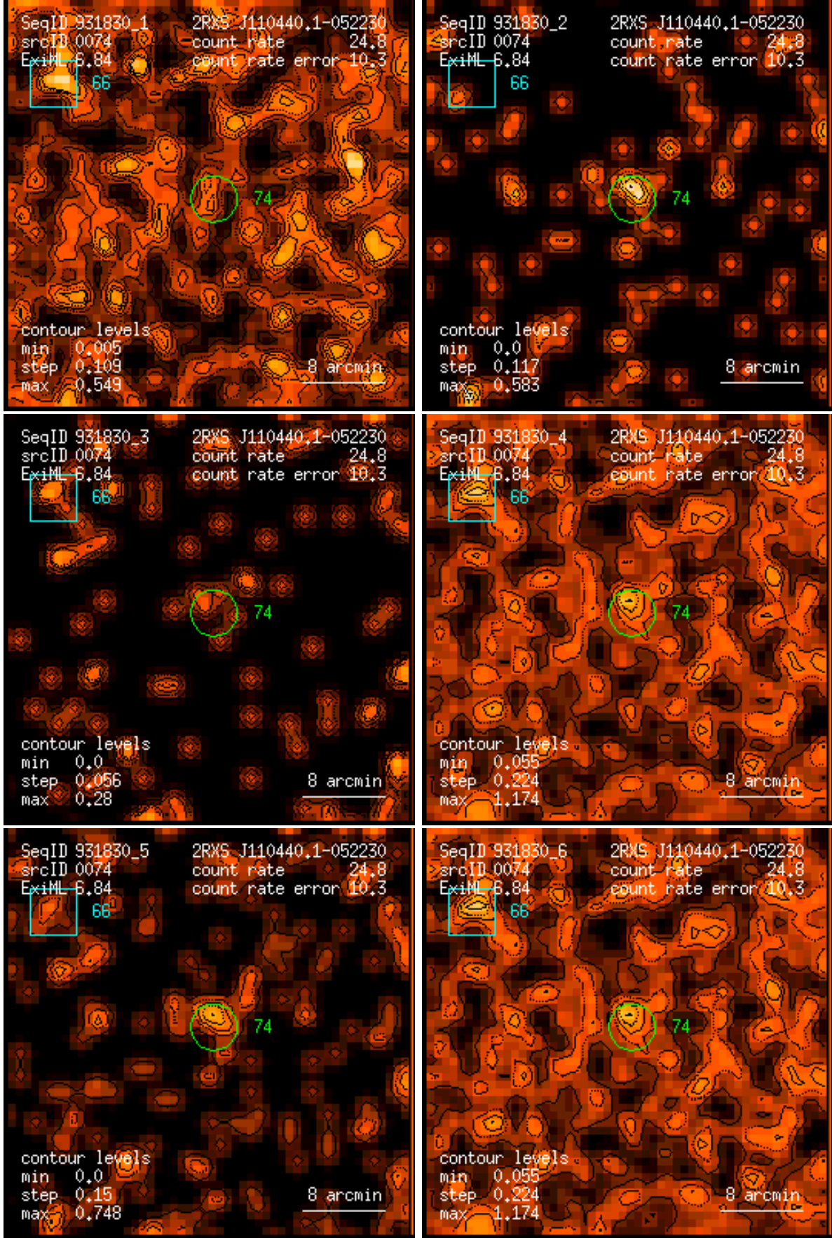
Figure 74: RASS 931830: detection 0074: band rate images, Gaussian filter: (1) PSPC channels 11 – 41, (2) 52 – 90, (3) 91 – 201, (4) 11 – 235, (5) 52 – 201, (6) 11 – 201. Broad band rates in counts/ks. Band rate contour levels in counts/ks/arcmin 2 .
