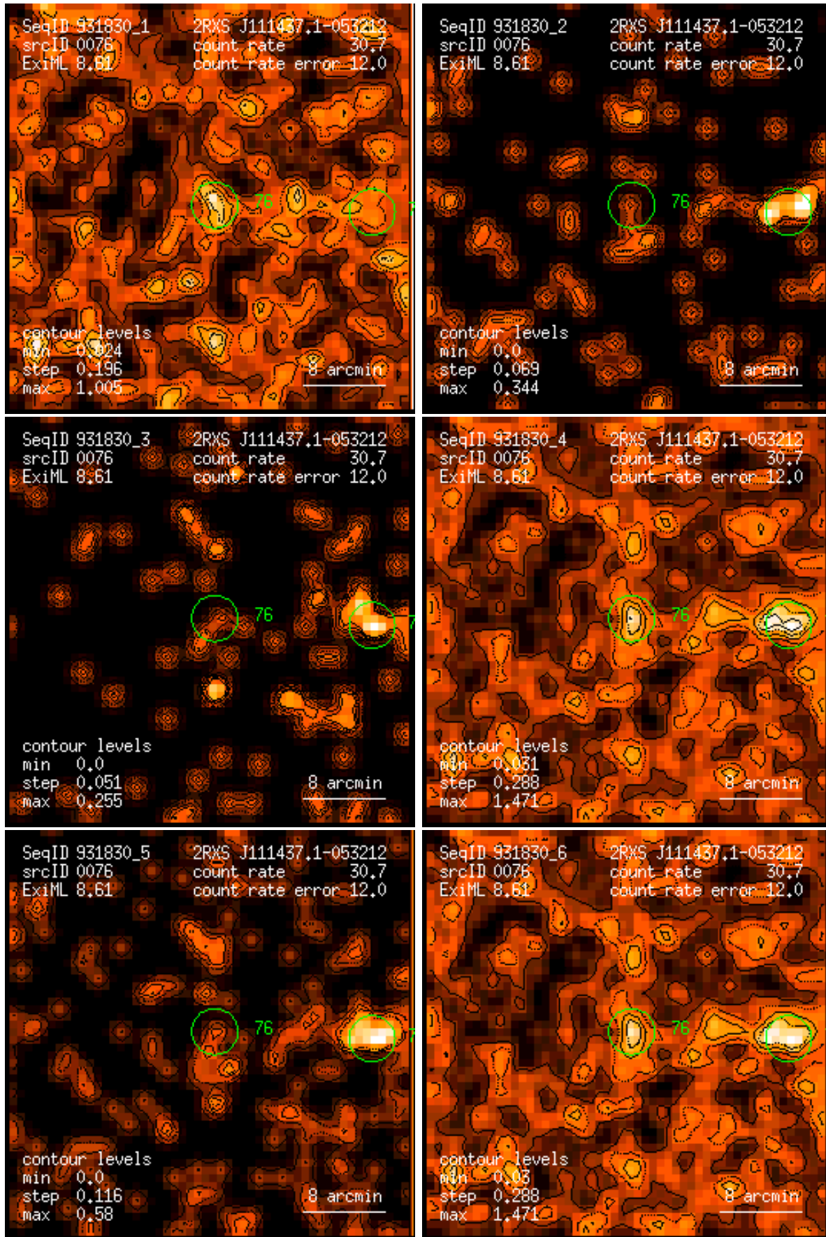
Figure 76: RASS 931830: detection 0076: band rate images, Gaussian filter: (1) PSPC channels 11 – 41, (2) 52 – 90, (3) 91 – 201, (4) 11 – 235, (5) 52 – 201, (6) 11 – 201. Broad band rates in counts/ks. Band rate contour levels in counts/ks/arcmin 2 .
