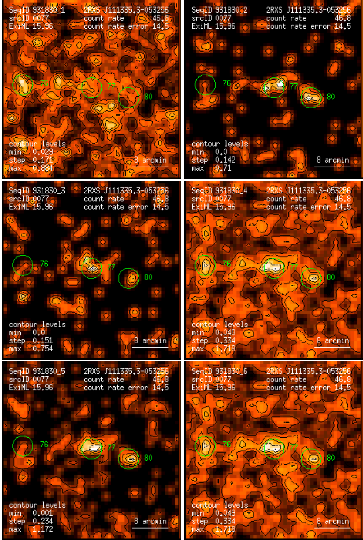
Figure 77: RASS 931830: detection 0077: band rate images, Gaussian filter: (1) PSPC channels 11 – 41, (2) 52 – 90, (3) 91 – 201, (4) 11 – 235, (5) 52 – 201, (6) 11 – 201. Broad band rates in counts/ks. Band rate contour levels in counts/ks/arcmin 2 .
