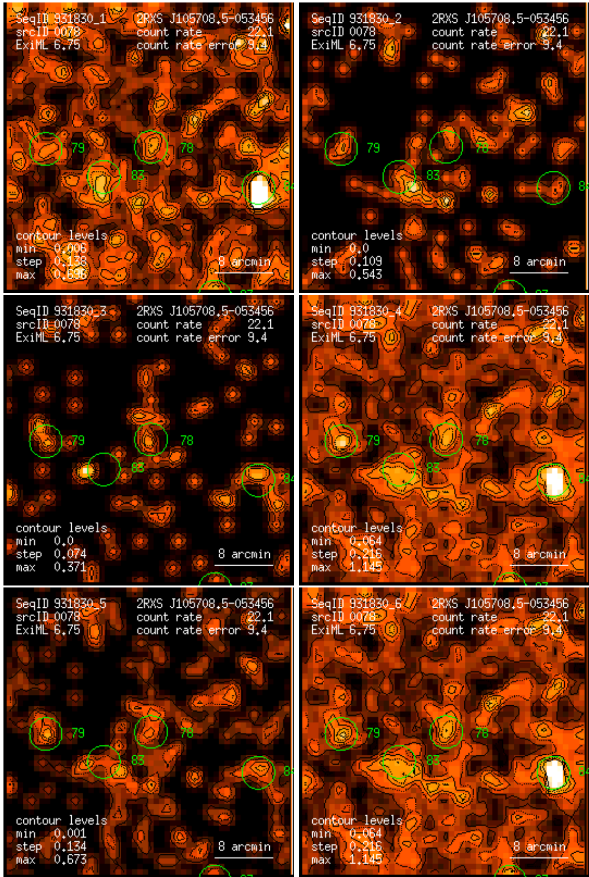
Figure 78: RASS 931830: detection 0078: band rate images, Gaussian filter: (1) PSPC channels 11 – 41, (2) 52 – 90, (3) 91 – 201, (4) 11 – 235, (5) 52 – 201, (6) 11 – 201. Broad band rates in counts/ks. Band rate contour levels in counts/ks/arcmin 2 .
