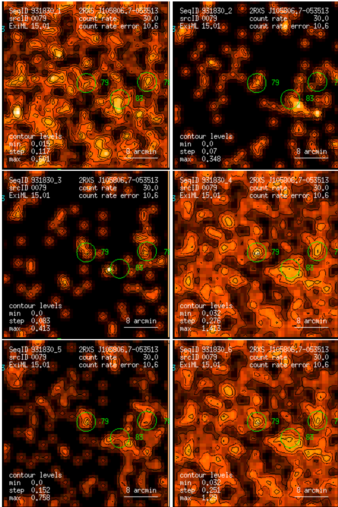
Figure 79: RASS 931830: detection 0079: band rate images, Gaussian filter: (1) PSPC channels 11 – 41, (2) 52 – 90, (3) 91 – 201, (4) 11 – 235, (5) 52 – 201, (6) 11 – 201. Broad band rates in counts/ks. Band rate contour levels in counts/ks/arcmin 2 .
