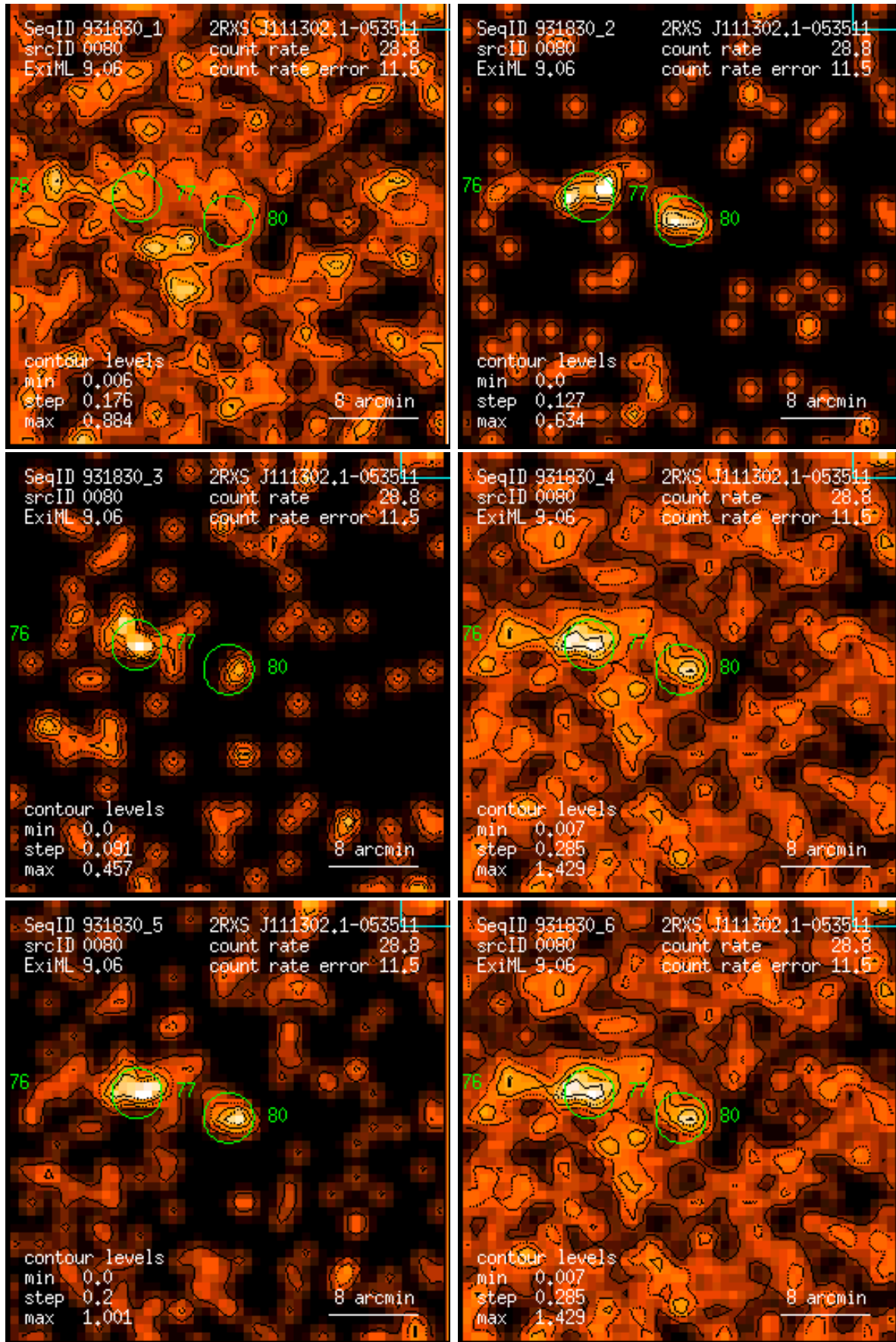
Figure 80: RASS 931830: detection 0080: band rate images, Gaussian filter: (1) PSPC channels 11 – 41, (2) 52 – 90, (3) 91 – 201, (4) 11 – 235, (5) 52 – 201, (6) 11 – 201. Broad band rates in counts/ks. Band rate contour levels in counts/ks/arcmin 2 .
