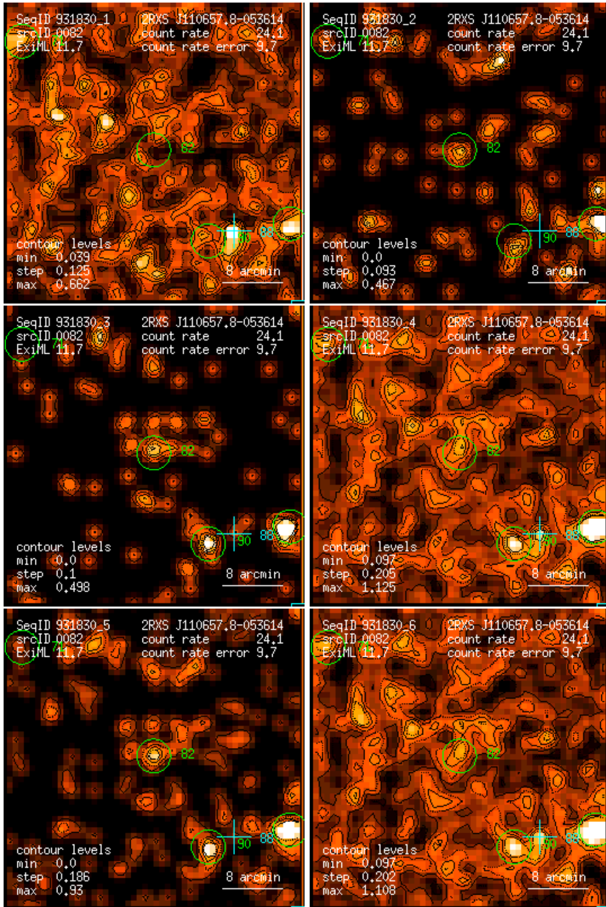
Figure 82: RASS 931830: detection 0082: band rate images, Gaussian filter: (1) PSPC channels 11 – 41, (2) 52 – 90, (3) 91 – 201, (4) 11 – 235, (5) 52 – 201, (6) 11 – 201. Broad band rates in counts/ks. Band rate contour levels in counts/ks/arcmin 2 .
