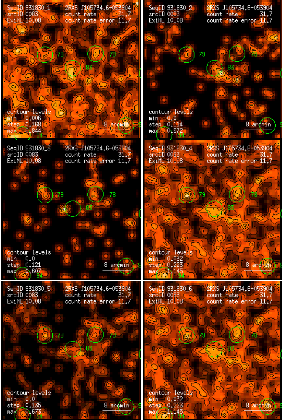
Figure 83: RASS 931830: detection 0083: band rate images, Gaussian filter: (1) PSPC channels 11 – 41, (2) 52 – 90, (3) 91 – 201, (4) 11 – 235, (5) 52 – 201, (6) 11 – 201. Broad band rates in counts/ks. Band rate contour levels in counts/ks/arcmin 2 .
