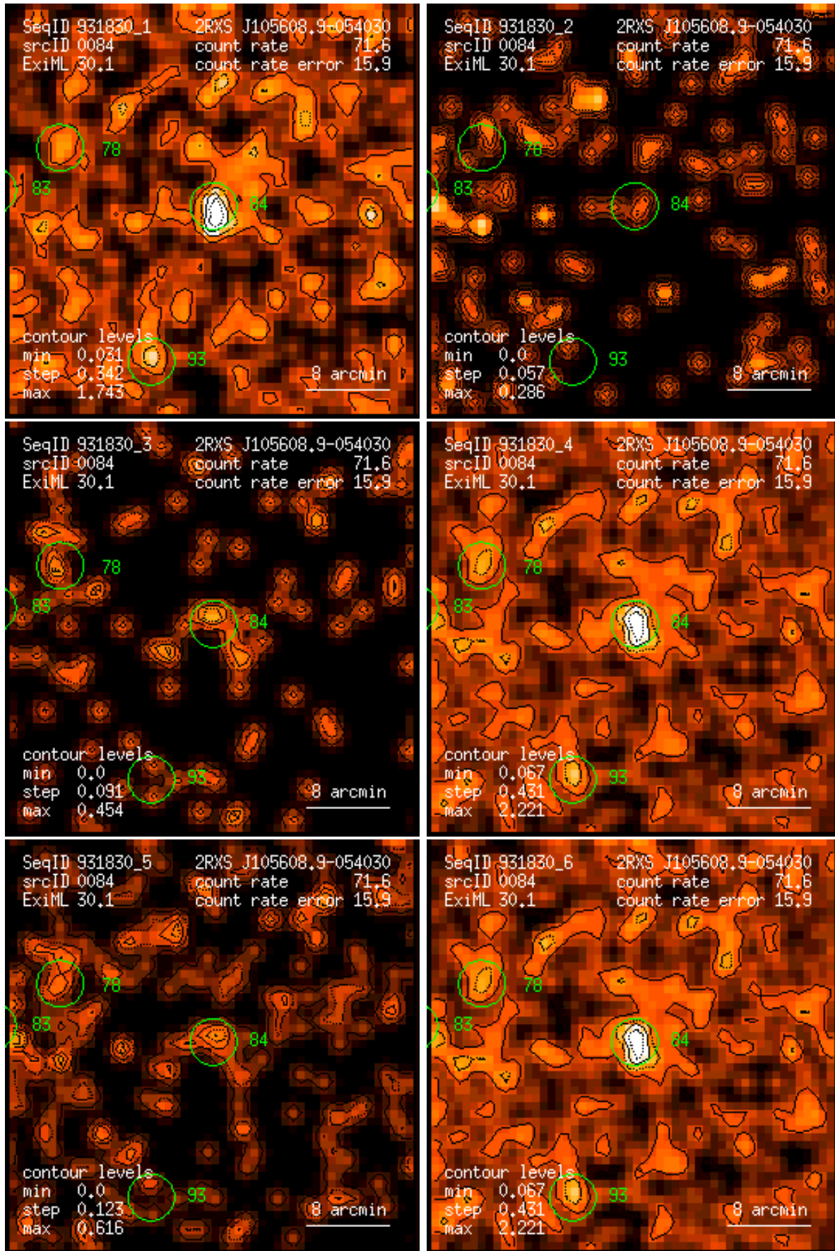
Figure 84: RASS 931830: detection 0084: band rate images, Gaussian filter: (1) PSPC channels 11 – 41, (2) 52 – 90, (3) 91 – 201, (4) 11 – 235, (5) 52 – 201, (6) 11 – 201. Broad band rates in counts/ks. Band rate contour levels in counts/ks/arcmin 2 .
